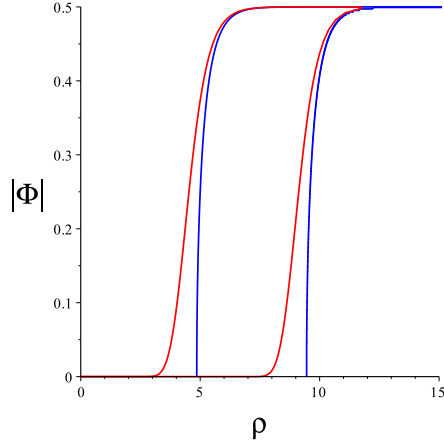
Figure 2: The red curves display the length of the Higgs field |\Phi| as a function of geodesic distance from the origin \rho , along an axis that is perpendicular to the symmetry axis of the axial hyperbolic N -monopole with N = 100 and N = 10000 . The blue curves show the corresponding magnetic disc approximation.
