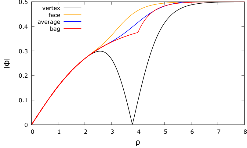
Figure 3: The length of the Higgs field, |\Phi| , for an icosahedrally symmetric strawberry flavour monopole with charge N = 371 . The plot shows |\Phi| as a function of geodesic distance from the origin \rho along a radial half-line that passes through a vertex (black curve) and a face centre (yellow curve) of the associated polyhedron. The blue curve is the spherical average of |\Phi| , obtained by integrating over the angular coordinates. The red curve is the new magnetic bag approximation.
