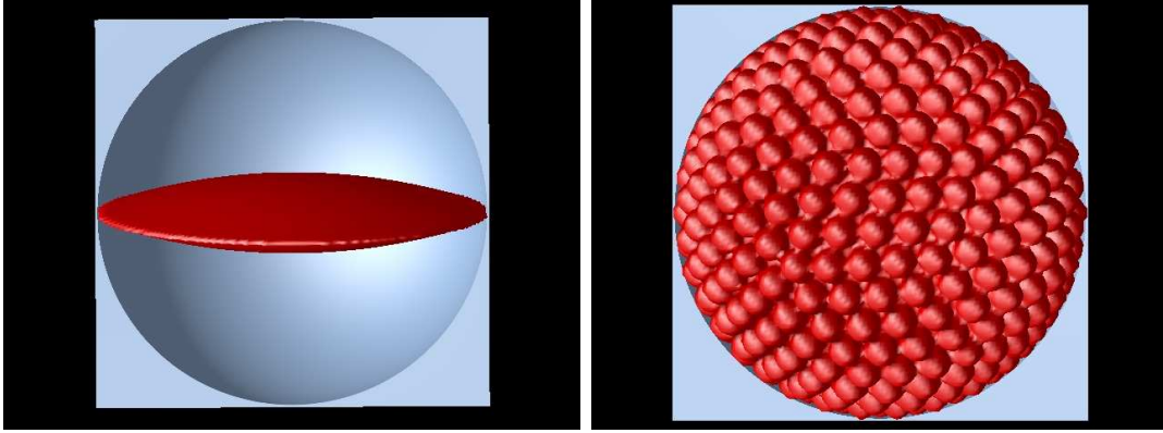
Figure 1: Energy density isosurfaces, in the ball model of \mathbb{H}^3 , for hyperbolic monopoles with N = 371 . The hyperbolic monopole in the left image has axial symmetry and is cherry flavour, whereas the one in the right image has icosahedral symmetry and is strawberry flavour. The blue sphere represents the boundary of hyperbolic space.
