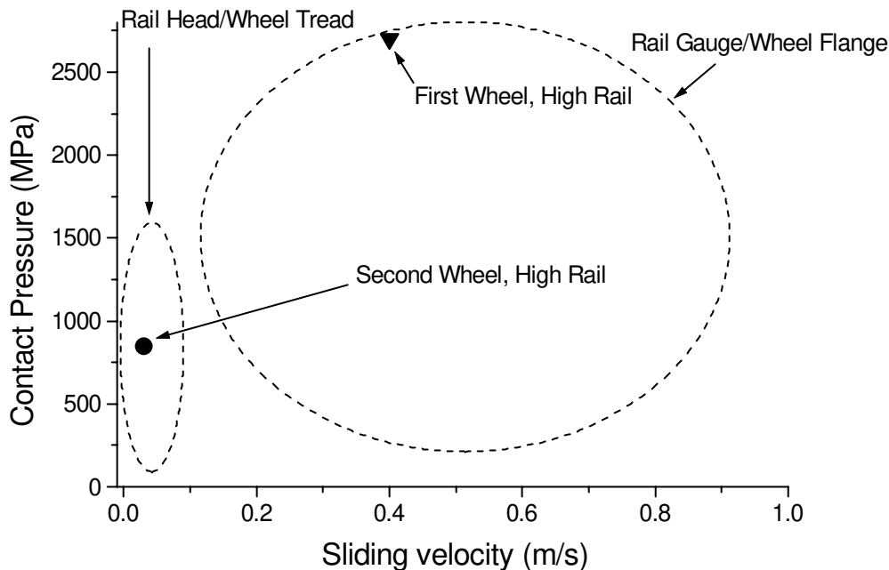
figure 9 Wheel/rail contact conditions on the Stockholm local railway network derived from GENSYS simulations [6] (also shown are results from Medyna simulations of the Älvsjö test track [16] for the first and second wheelsets)
