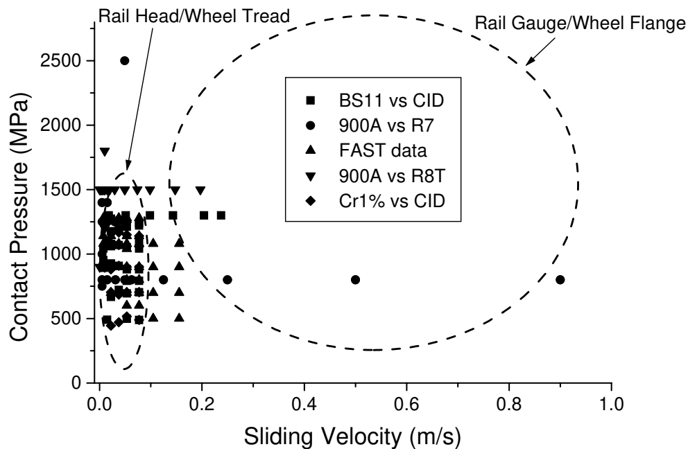
figure 11 Available rail steel wear data plotted over typical wheel/rail contact conditions
