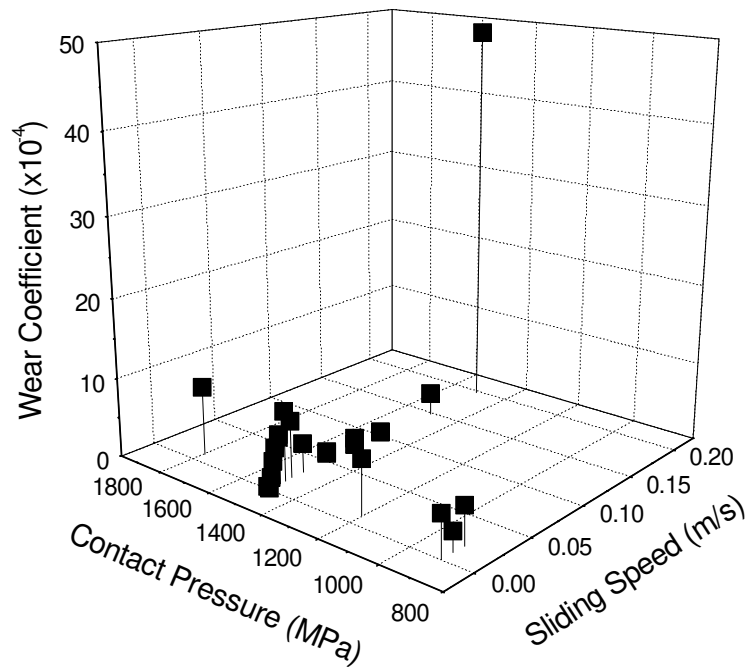
figure 8 Wear coefficient map for UIC60 900A versus R8T wheel material
