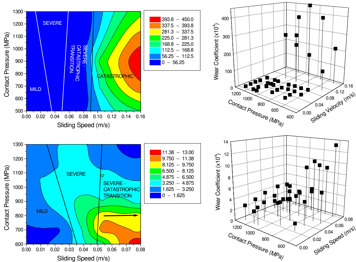
figure 6 Wear coefficient maps for standard carbon rail material and an unspecified wheel material (data from [9])
