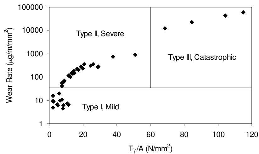
figure 1 Wear regimes identified during twin disc testing of BS11 rail material versus Class D tyre material [5]
