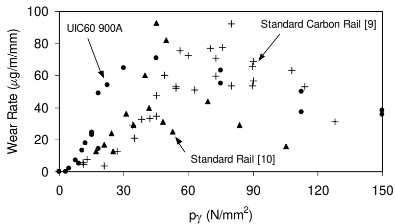
figure 3 Total wheel and rail wear rate in the heavy wear regime
