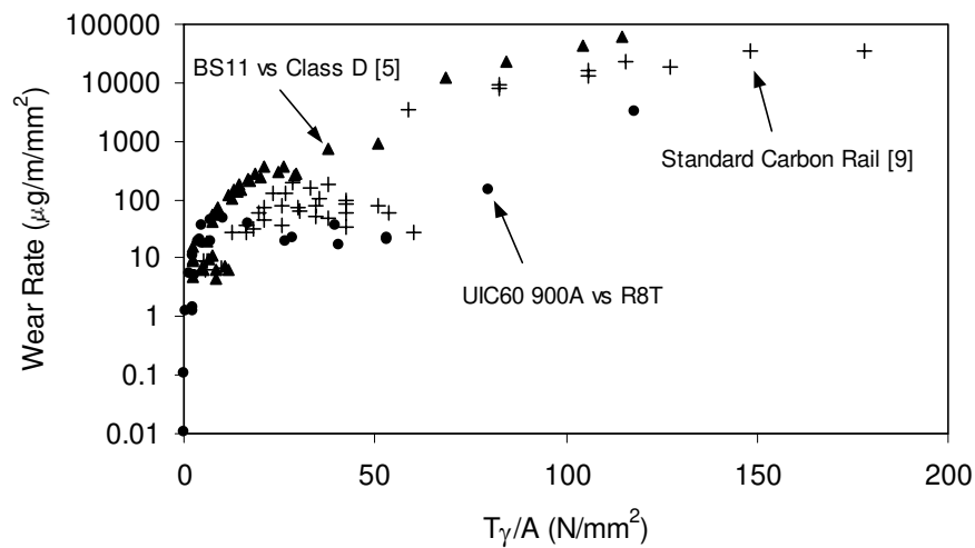
figure 2 Wear rates resulting from twin disc testing for a number of different material combinations
