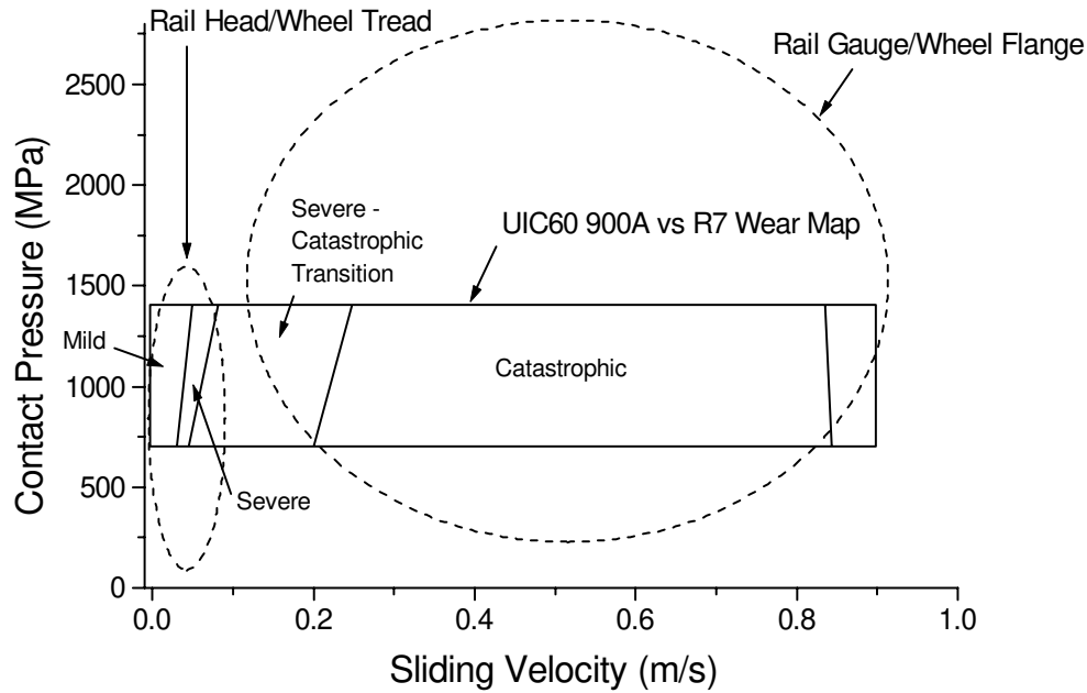
figure 10 UIC60 900A rail steel wear map plotted over wheel/rail contact conditions derived from GENSYS simulations [6]
