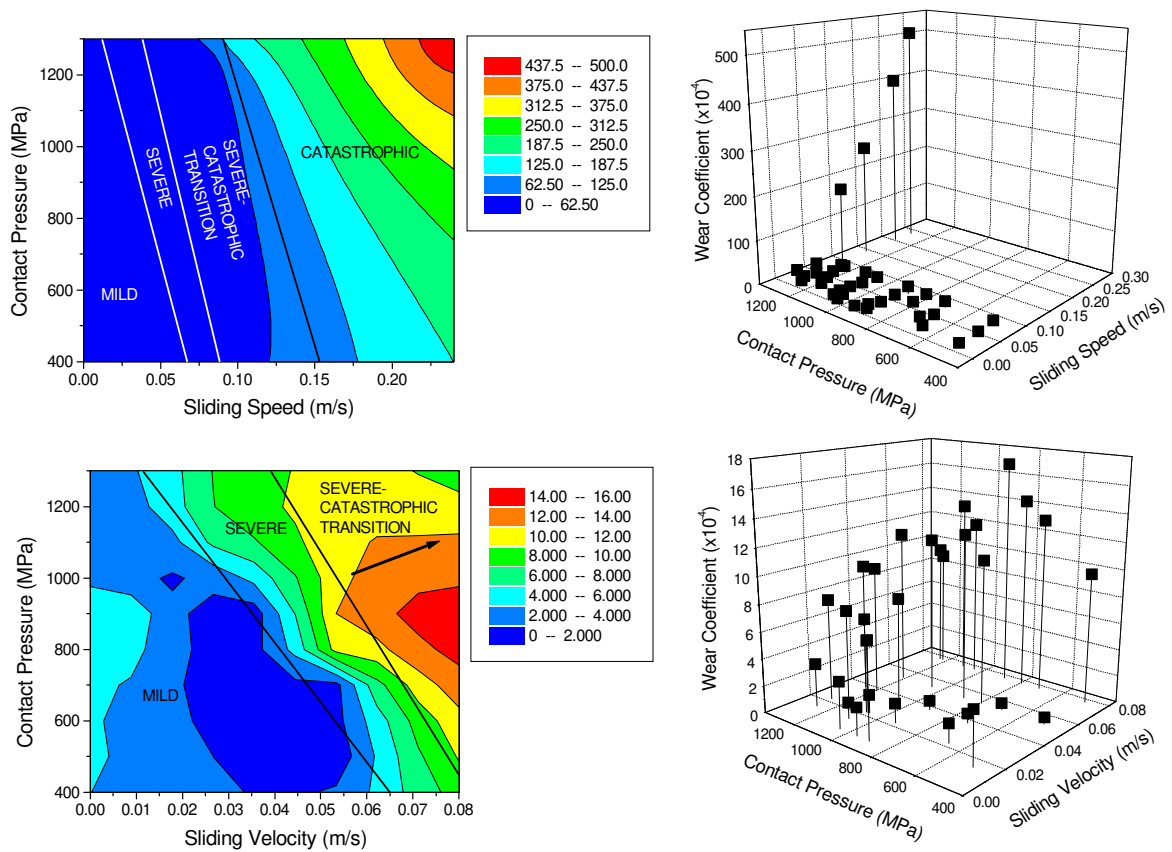
figure 5 Wear coefficient maps for BS11 rail material versus Class D tyre material (data from [5])
