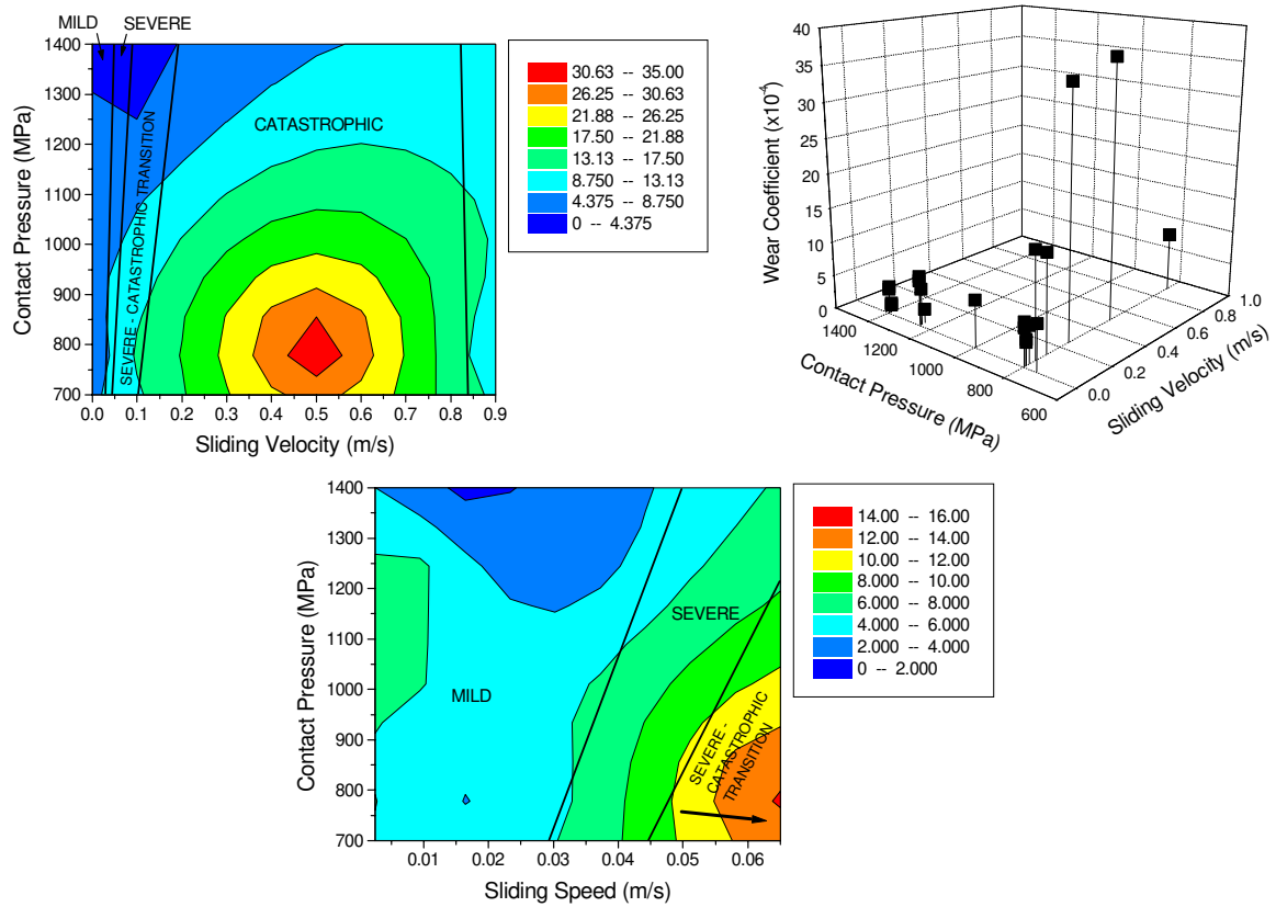
figure 7 Wear coefficient maps for UIC60 900A rail material versus R7 wheel material (data from [3])
