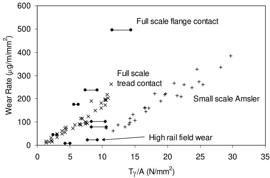
figure 4 Comparison of rail wear data from small and full-scale laboratory tests and the field [11]
