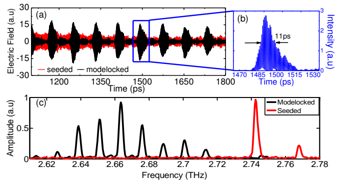
Fig. 1. Active modelocking of the metal-metal QCL at 77K. (a) Output electric field for the seeded (red) and the modelocked (black) QCL. (b) Expanded view of the THz pulse intensity between 1470ps and 1530 ps. (c) FFT of figure (a) for seeded (red) and modelocked (black) QCL.
