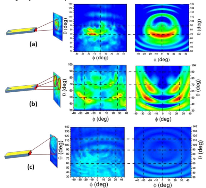
Fig. 1. Simulated far-field patterns (right side) of metal-metal THz QCLs and their corresponding far-field patterns measured at 77K (left). (a) 40 \mu m-wide metal-metal THz QCL (b) 80 \mu m-wide metal-metal THz QCL. (a) and (b) are with \sim 150 \mu m-long planar horn antennas integrated onto QCL top metal at both side of the facet. (c) 60 \mu m-wide metal-metal THz QCL without any planar horn antenna.
