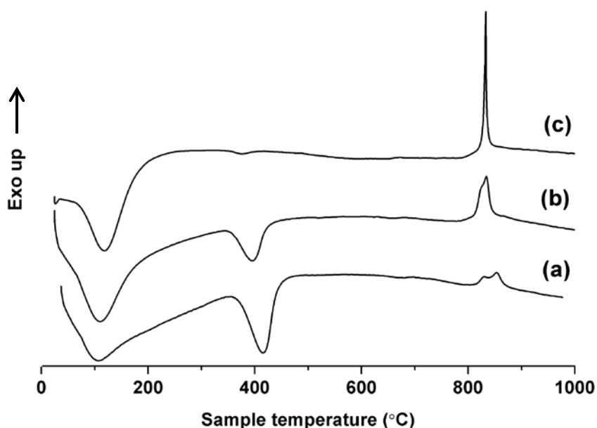
Figure 7. DTA data for 1:1 \text{Mg}(\text{OH})_2\text{:SiO}_2 (w/b = 1.0) with 2 wt.% (\text{NaPO}_3)_6 , at curing ages of (a) 7, (b) 14 and (c) 28 days
