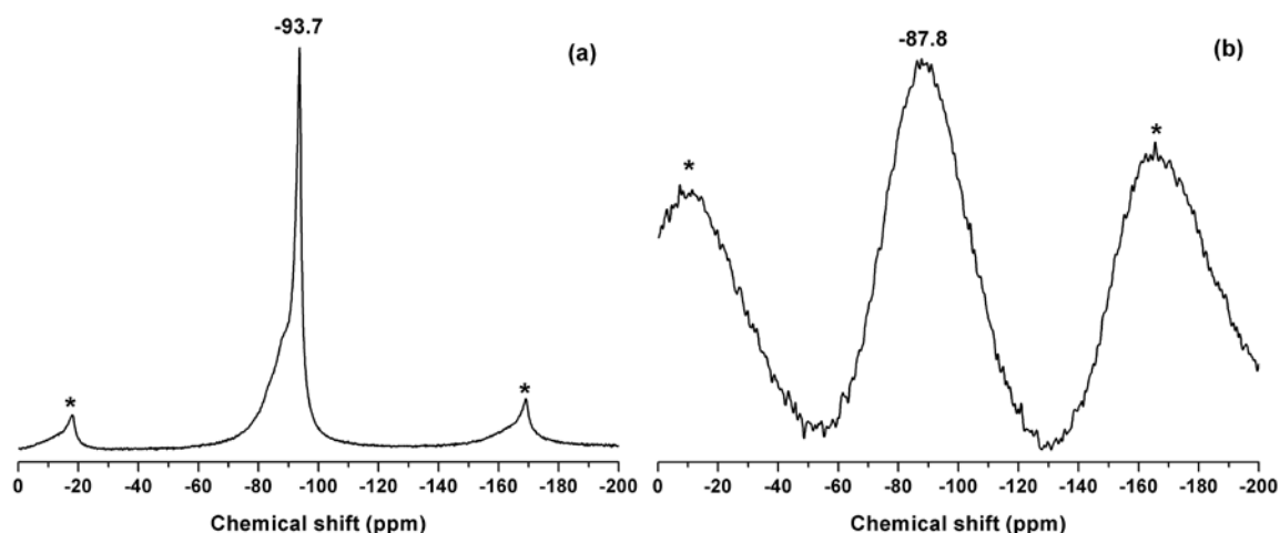
Figure 11. ^{29}Si MAS NMR spectra for: (a) lizardite, (b) antigorite. Spinning sidebands marked with *
