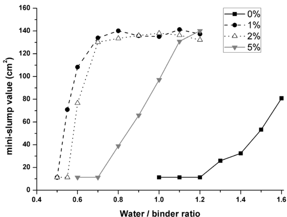
Figure 1. Mini-slump values for 1:1 Mg(OH)_2:SiO_2 with 0-5 wt.% (NaPO_3)_6 as shown in the legend, as a function of water/binder ratio. A measurement of 11.3\text{ cm}^2 indicates no slump, as this is the initial slump cone area
