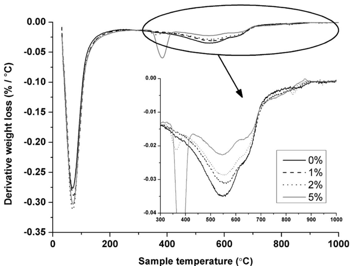
Figure 4. DTG data for 1:1 Mg(OH)_2 : SiO_2 (w/b = 1.0) with 0 – 5 wt.% (NaPO_3)_6 , samples cured for 28 days. Inset shows the data above 300 °C with an expanded vertical scale
