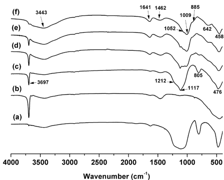
Figure 9. FTIR spectra of (a) silica fume, (b) Mg(OH)_2 , (c) 1:1 Mg(OH)_2:SiO_2 with 2 wt.% (NaPO_3)_6 as an anhydrous powder mix, and hydrated samples cured for (d) 7, (e) 14 and (f) 28 days (w/b = 1.0 for all hydrated samples)
