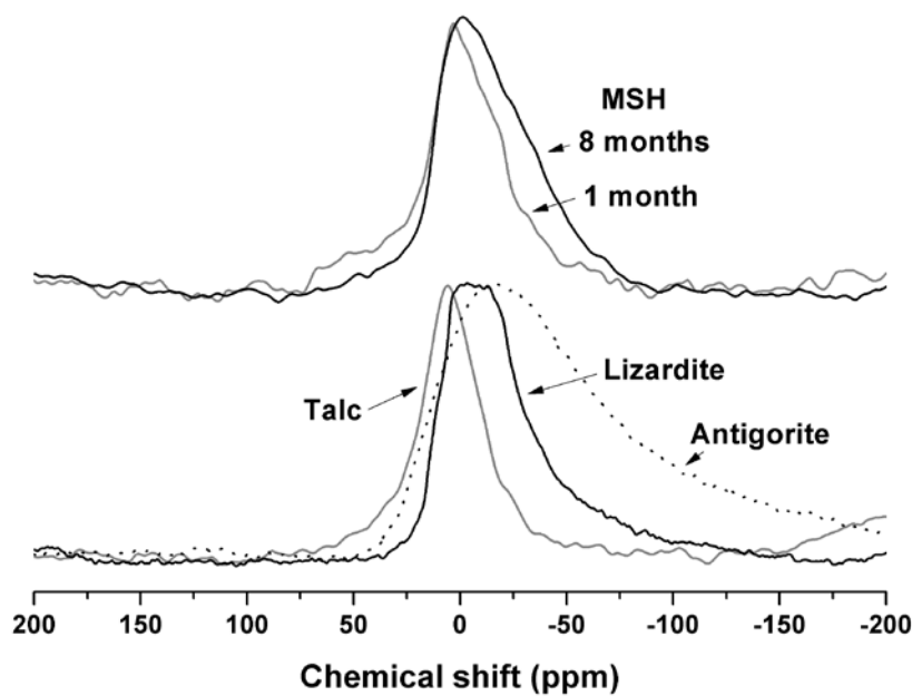
Figure 12. ^{25}Mg MAS NMR spectra of 1 and 8 month cured M-S-H with reference materials.
