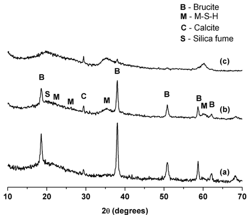
Figure 5. X-ray diffractograms of 1:1 Mg(OH)_2:SiO_2 (w/b = 1.0) with 2 wt.% (NaPO_3)_6 at curing ages of (a) 7, (b) 14 and (c) 28 days
