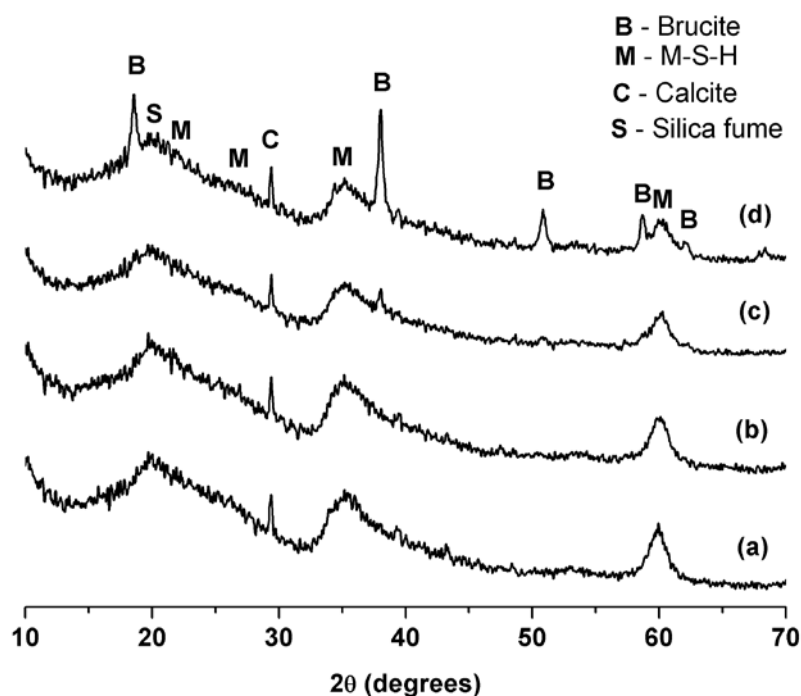
Figure 3. X-ray diffraction patterns of 28 day-cured 1:1 Mg(OH)_2:SiO_2 ( w/b = 1.0 ) binders, with (a) 0, (b) 1, (c) 2 and (d) 5 wt.% (NaPO_3)_6 addition
