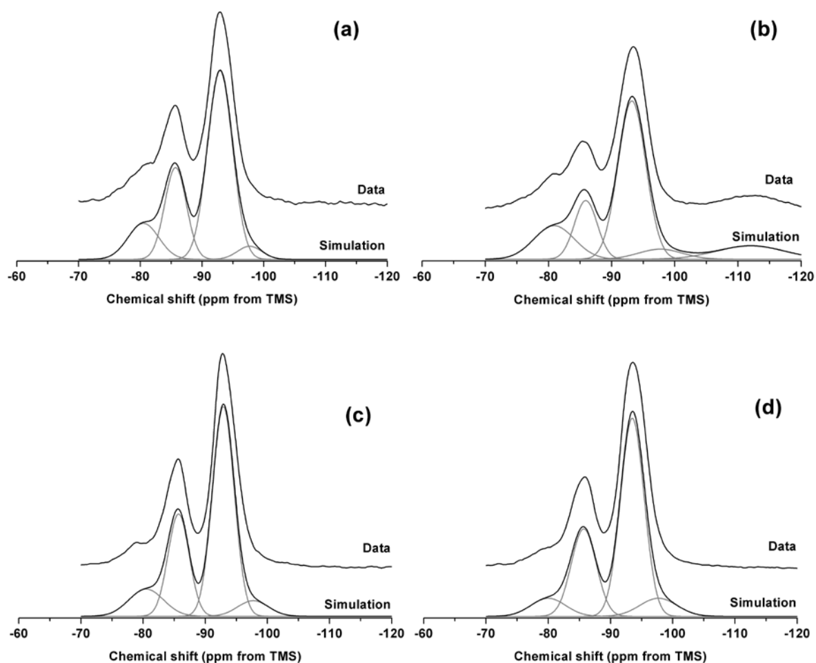
Figure 10. ^{29}Si MAS NMR spectra for 1:1 Mg(OH)_2:SiO_2 (w/b 1.0) with (a) 0 and (b) 2 wt. % (NaPO_3)_6 at a curing age of 1 month, (c) 0 and (d) 2 wt. % (NaPO_3)_6 after 8 months of curing. The data presented include a simulation and constituent peaks underneath.
