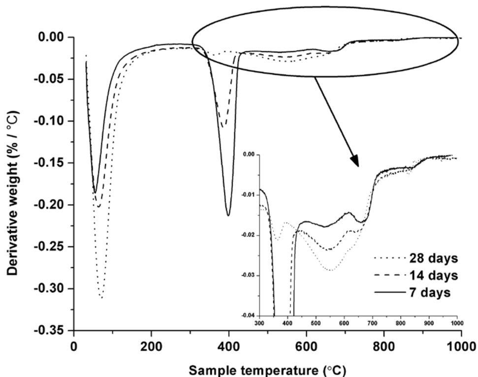
Figure 6. DTG data for 1:1 Mg(OH)_2:SiO_2 ( w/b = 1.0 ) with 2 wt.% (NaPO_3)_6 , at curing ages of 7, 14 and 28 days
