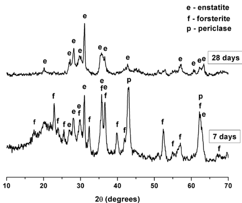
Figure 8. XRD patterns of 1:1 \text{Mg}(\text{OH})_2\text{:SiO}_2 ( w/b = 1.0 ) heated to 900^\circ\text{C} after 7 and 28 days of curing
