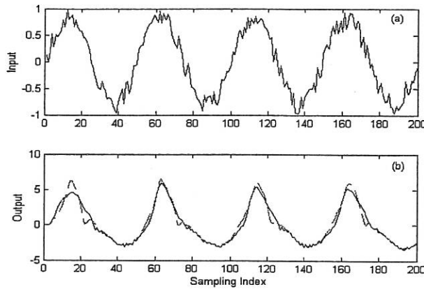
Figure 4 Performance of the identified model (28) for the TARSO system (26) by setting the input signal u(t) = u_1(t) + w_1(t) , where u_1(t) = 0.8 \sin(2\pi t / 50) and w_1(t) was a random sequence uniformly distributed in [-0.2, 0.2] . (a) The input. (b) A comparison between the recovered signal from the model (28) and the output from the original system (26). (The solid line in (b) indicates the real output, and the dashed line indicates the simulated output from the identified model (28)).
