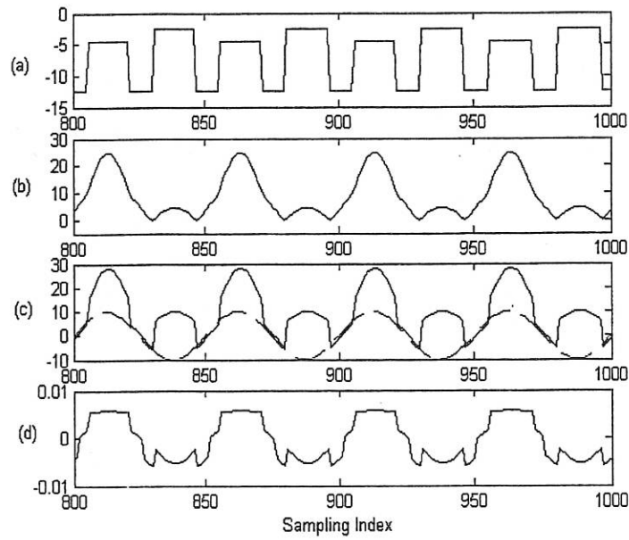
Figure 3 Signals recovered from f^{[1]} , f^{[2]} and f^{[1]} + f^{[2]} based on the model (25). (a) Recovered from f^{[1]} ; (b) Recovered from f^{[2]} ; (c) A comparison between the signal recovered from f^{[1]} + f^{[2]} and the that from the original system (22). (d) The discrepancy between the recovered signal from (25) and that from the original system (22).
