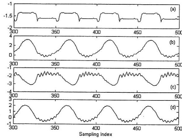
Figure 9 Signals recovered from f^{[1]} , f^{[2]} , f^{[4]} and f^{[1]} + f^{[2]} + f^{[4]} based on the model (32). (a) Recovered from f^{[1]} . (b) Recovered from f^{[2]} . (c) Recovered from f^{[4]} . (d) Superimposition f^{[1]} + f^{[2]} + f^{[4]} .
