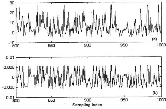
Figure 2 A comparison between the model predicted output from the model (25) and the that from the original system (22) with the input as a random sequence. (a) Overlap of the outputs from (22) and (25); (b) The discrepancy between the outputs.
