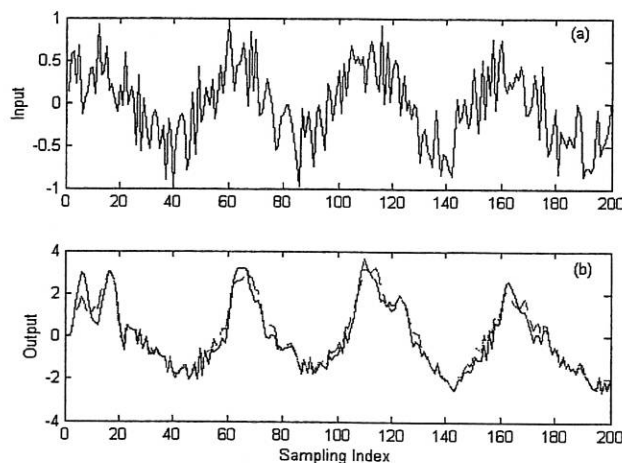
Figure 5 Performance of the identified model (28) for the TARSO system (26) by setting the input signal u(t) = u_2(t) + w_2(t) , where u_2(t) = 0.5 \sin(2\pi t / 50) and w_2(t) was a random sequence uniformly distributed in [-0.5, 0.5] . (a) The input. (b) A comparison between the recovered signal from the model (28) and the output from the original system (26). (The solid line in (b) indicates the real output, and the dashed line indicates the simulated output from the identified model (28)).
