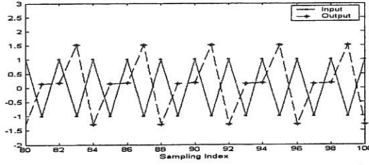
Figure 7 The HHARX system (31) is subharmonic driven by the input u(t) = (-1)^t
