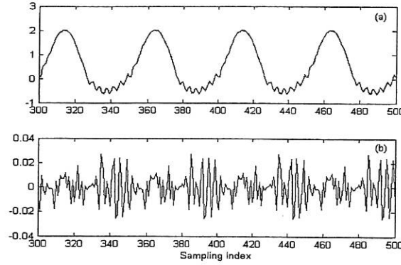
Figure 8 Performance of the identified model (32) over the test data set for the HHARX system (31). (a) Overlap of the output based on the model (32) and the measurements. (b) Discrepancy between the model predicted output and the measurements.
