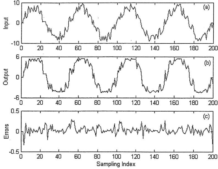
Figure 6 Performance of the identified model (30) for the TARSO system (29) by setting the input signal u(t) = u_1(t) + u_2(t) , where u_1(t) = 7.5 \sin(2\pi t / 50) and u_2(t) was a random sequence uniformly distributed in [-2.5, 2.5] . (a) The input. (b) A comparison between the recovered signal from the model (30) and the output from the original system (29). (The solid line in (b) indicates the real output, and the dashed line indicates the simulated output from the identified model (30)). (c) Model predicted errors.
