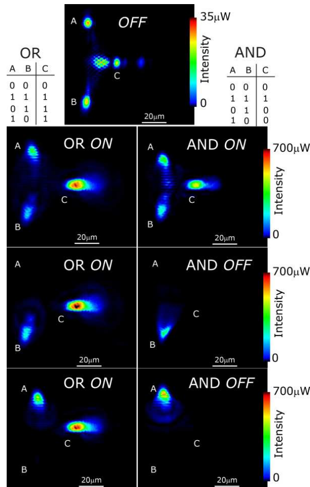
Fig. 4: Three transistors scheme (A,B and C, spatially separated by a distance of about 30 μm) in which C acts as AND/OR logic gate with inputs A and B. When A, B and C are below threshold as in (a), their output intensities are lower than 35 μW. The interference pattern originated by the three fluids is visible near the intersection point in this low density regime. Due to the increase of the intensities above threshold, the color scales in panels (b,c,d,e,f,g) are reduced by a factor 20 as compared with panel (a). The OR gate is described in the left column with both A and B on (b), B only on (c), A only on (d). C is always activated when A or B or both are on. The AND gate is obtained by lowering 10% the Address power of C, and it is described in the right column with both A and B on (e), B only on (f), A only on (g). It is required that both A and B are on to activate C. The corresponding logic tables are resumed on top of each column.
