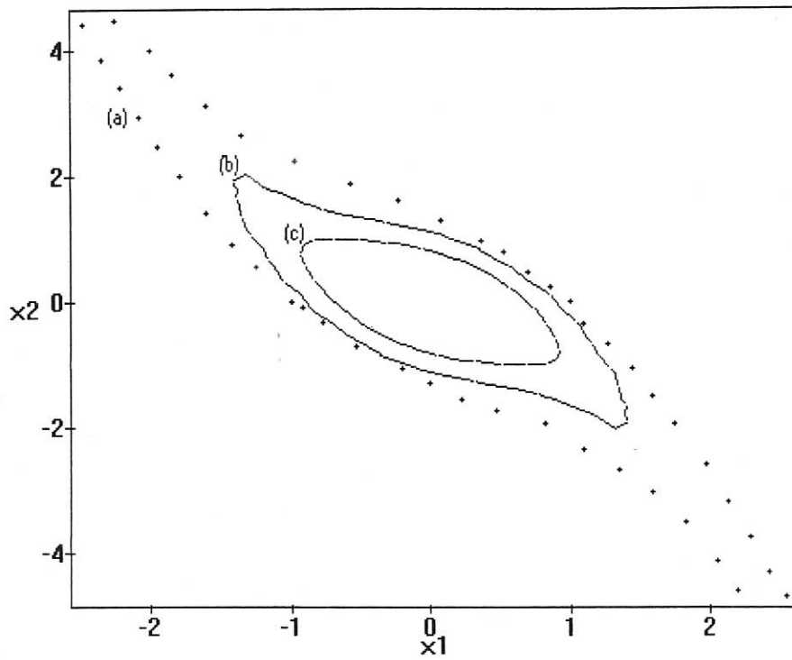
Approximations to a Lyapunov function for the above system
