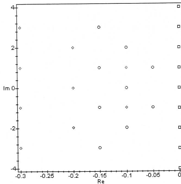
Root Locus with beta = 0, -0.1, -0.2
