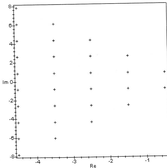
Poles of the Time-Reversed Van der Pol Oscillator
