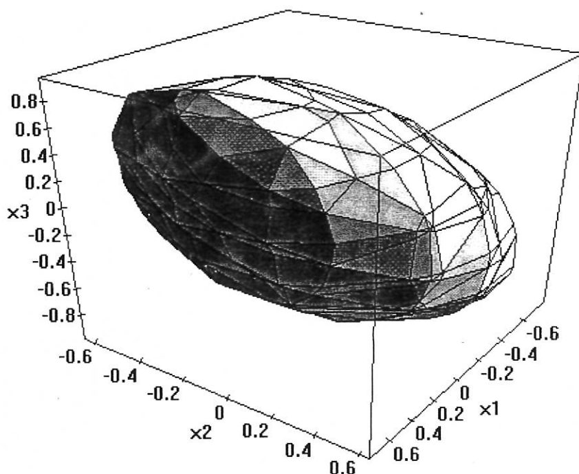
Approximate domain of attraction for a third order system
