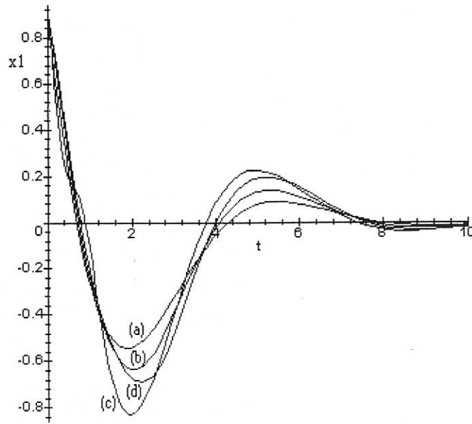
Approximations to the Solution
