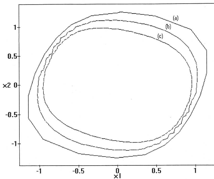
Approximate Lyapunov functions for inverse Van del Pol
