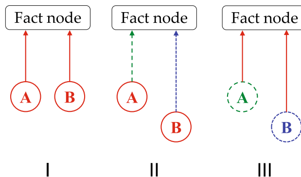
Fig. 3 The importance of the frame of reference in analyzing synchrony of activation. In situation I, two source nodes ( A , B ) are in synchrony ( red , unbroken lines ) in an outside frame of reference. They are also in synchrony in the frame of reference of the target ( Fact ) node, because their activation arrives in synchrony ( red , unbroken lines ). In situation II, A and B are in synchrony in the outside frame of reference ( red , unbroken lines ), but not in the frame of reference of the Fact node, because their activation does not arrive in synchrony ( green and blue , dashed lines ). In situation III, A and B are in not synchrony in the outside frame of reference ( green and blue , dashed lines ), but they are in synchrony in the frame of reference of the Fact node, because their activation arrives in synchrony ( red , unbroken lines ). (Color figure online)
