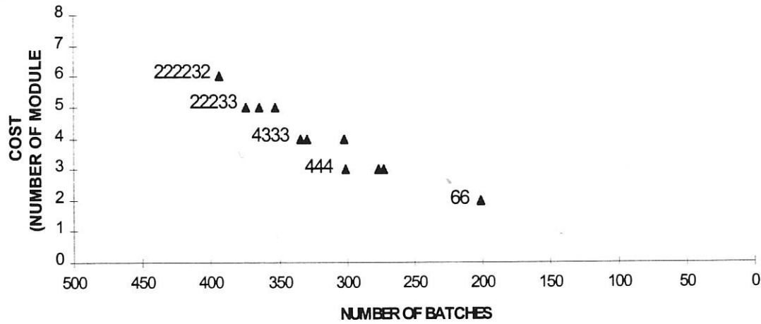
Figure 9 : MOGA approach
