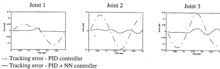
Fig. 3. Tracking errors from each joint.
