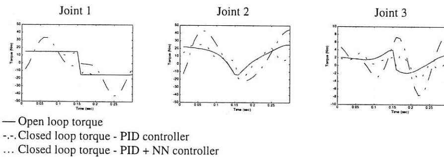
Fig. 4. Open-loop torque and closed-loop torque on each joint.
