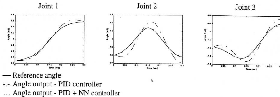
Fig. 2. Angular positions from each joint.
