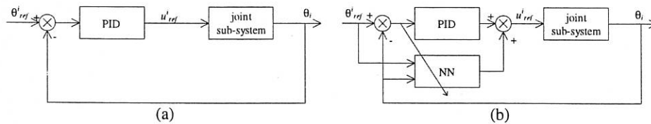
Fig. 1. (a) Independent joint controls using de-coupled control scheme. (b) Neural network and PID controllers in de-coupled control scheme.
