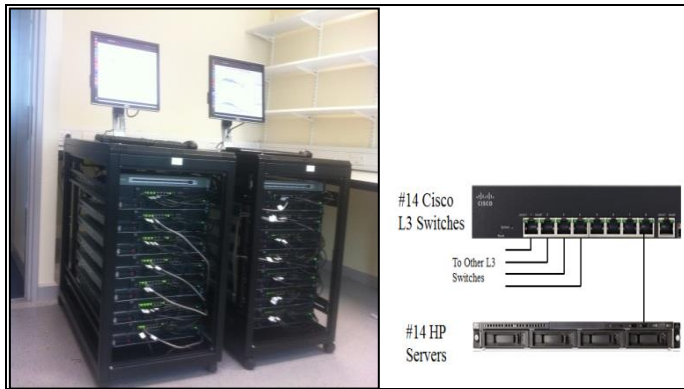
Fig. 15 Experiment Racks and Connectivity
