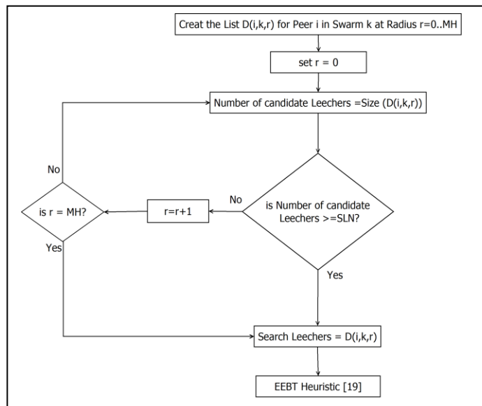
Fig. 9 The Flowchart of the EEBTv2 Heuristic
