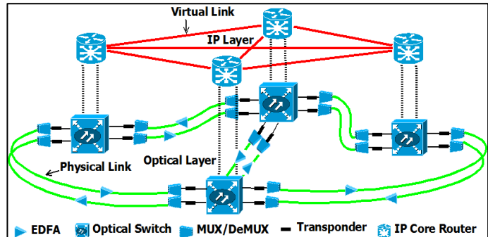
Fig. 1 IP/WDM Network
