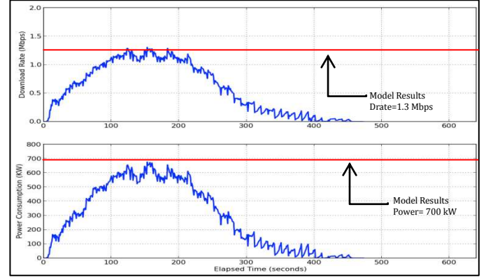
Fig. 16 Experimental Average Download Rate and IP/WDM Power Consumption of Original BitTorrent (OBT)
