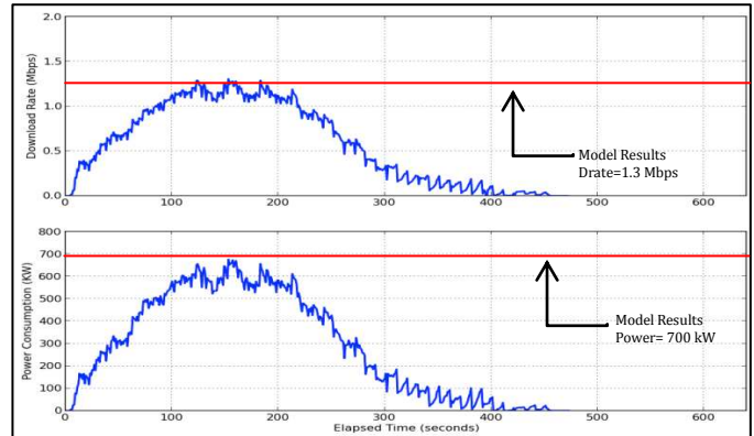
Fig. 16 Experimental Average Download Rate and IP/WDM Power Consumption of Original BitTorrent (OBT)
