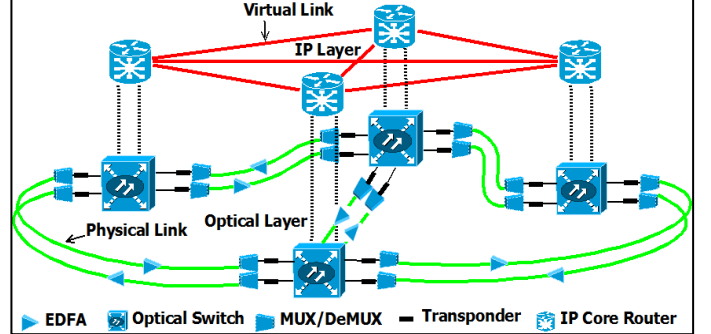
Fig. 1 IP/WDM Network
