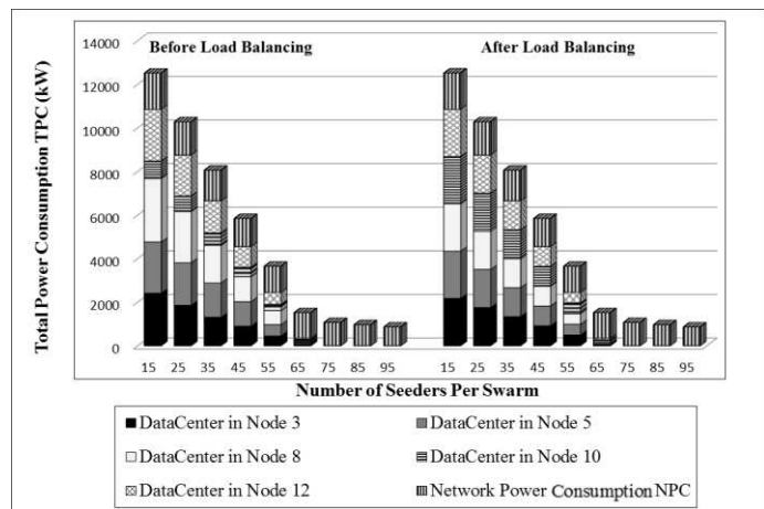
Fig. 14 Total Power Consumption (IP/WDM and Data Centers) With and Without Load Balancing in CDN-P2P
