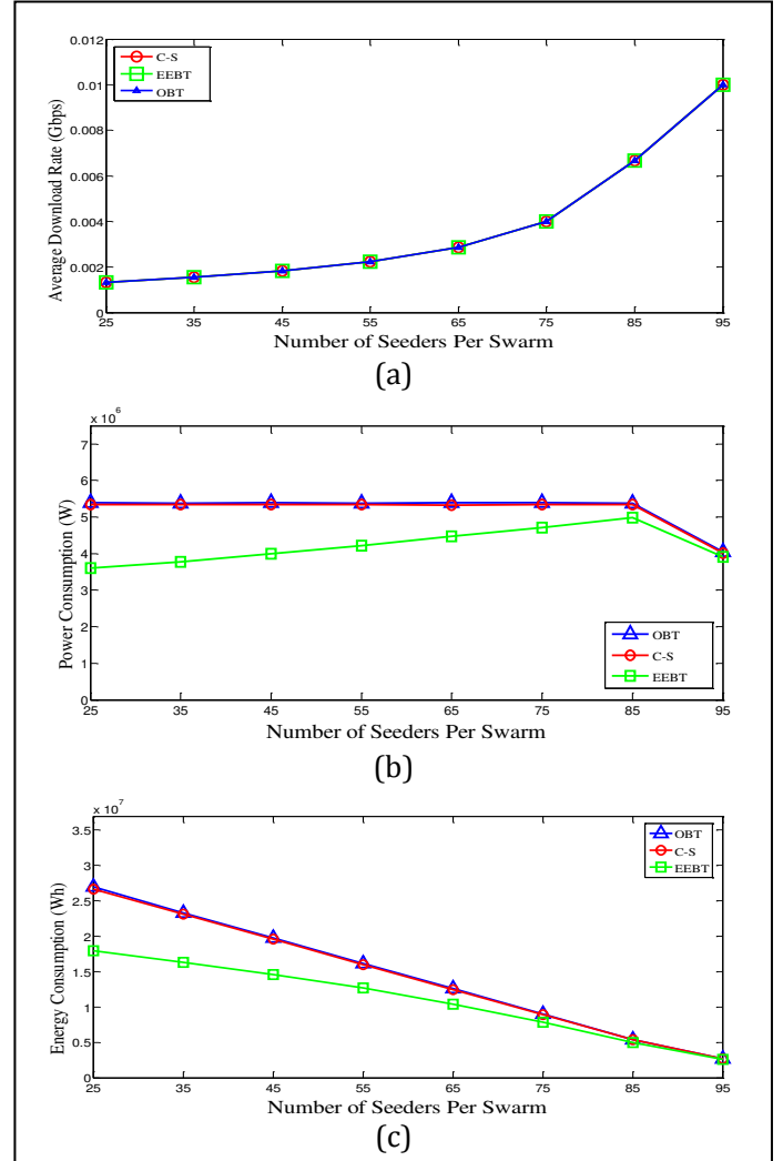
Fig. 4 AT&T Network Results (a) Download rate (b) IP/WDM Power Consumption (c) IP/WDM Energy Consumption
