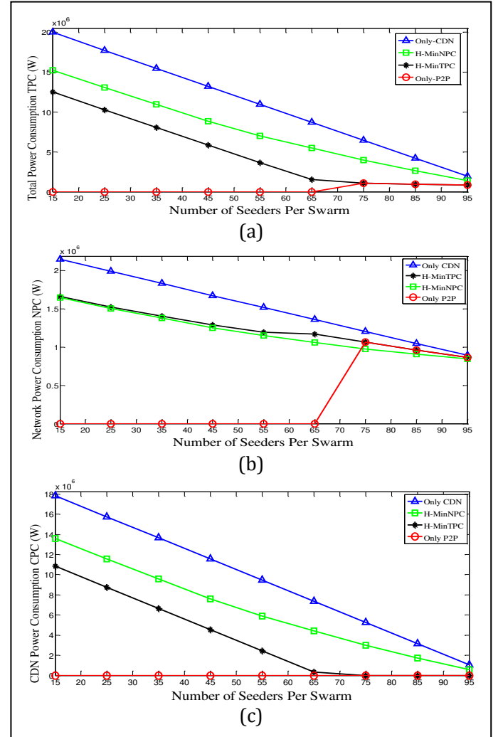
Fig. 12 CDN-P2P Results (a) Total Power Consumption (b) IP/WDM Network Power Consumption (c) CDN Datacenter Power Consumption
