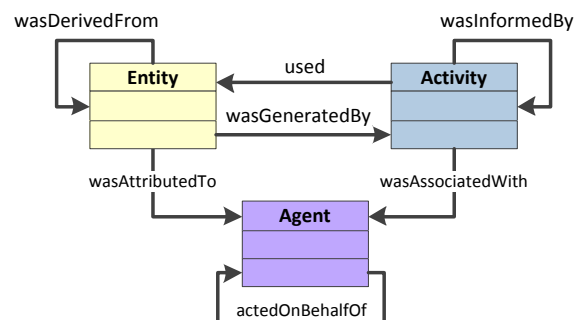
Figure 2: PROV Core Structures
