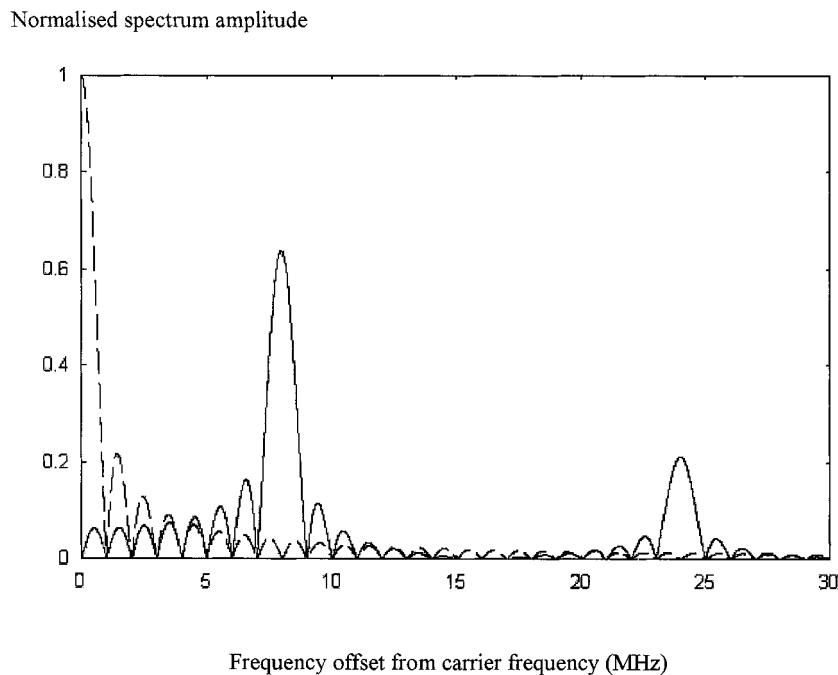
Fig. 7. One-sided frequency spectrum of pulsed carrier signal incident on and reflected from PSS switched at 8 MHz ( f_c = 10 GHz, 1 \mu s pulses, 1% pulse duty cycle) (--- Incident signal, — Reflected signal).
