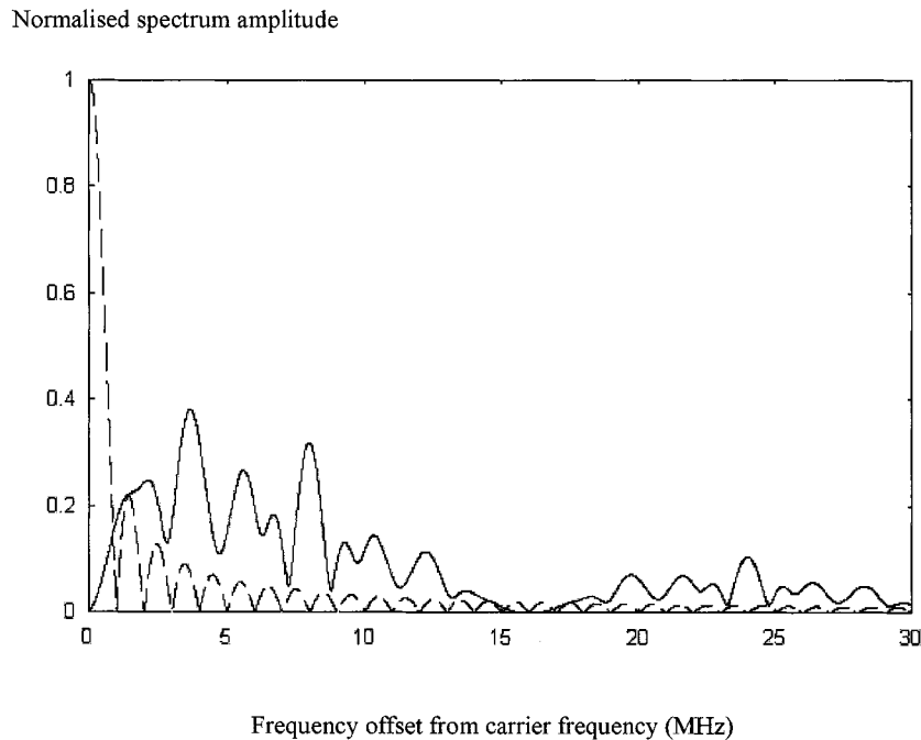
Fig. 9. One-sided frequency spectrum of pulsed carrier signal incident on and reflected from PSS switched at 8 MHz using a sequence derived from the primitive polynomial modulo 2 (4, 1, 0), f_c = 10 GHz, 1- \mu s pulses, 1% duty cycle (--- Incident signal, — Reflected signal).
