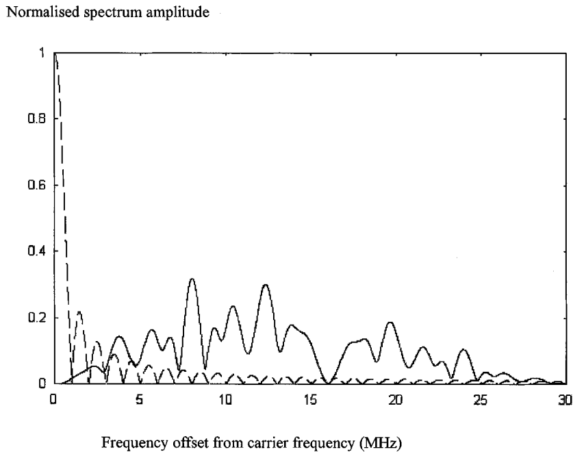
Fig. 10. As Fig. 9 but with additional Manchester encoding (--- Incident signal, — Reflected signal).
