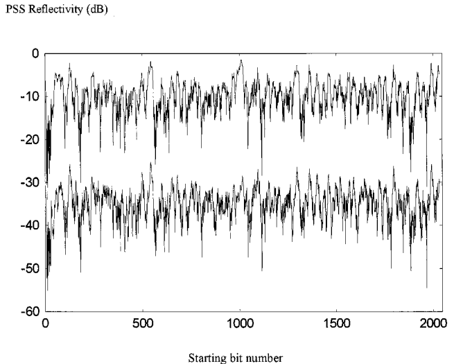
Fig. 13. Variation in PSS reflectivity as the 16-b switching sequence contained within the width of a 1- \mu s radar pulse is chosen sequentially from an overall switching sequence of 2048 b. Top curve = bipolar switching based directly on the bit sequence generated by an 11th-order polynomial (modulo 2). Mean reflectivity value = -10.2 dB. Bottom curve = as top curve, but when Manchester encoding is used. Mean reflectivity value = -35.1 dB.
