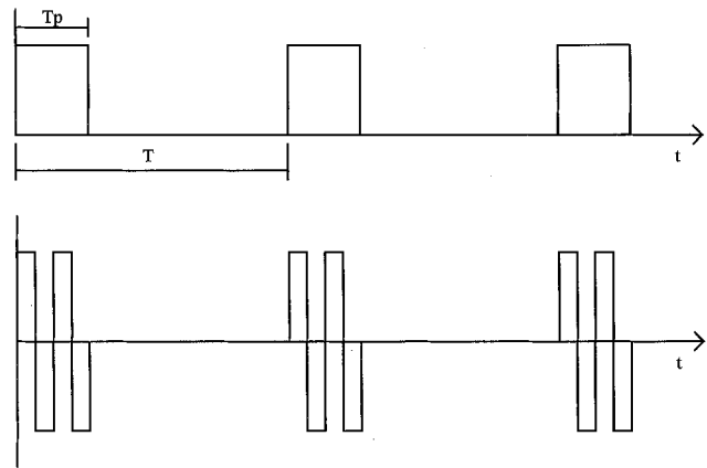
Fig. 3. Operation of the phase switched screen, (a) incident wave, (b) reflected wave ( M = 2 . For clarity, the sinusoidal carrier frequency signal itself is not shown).
