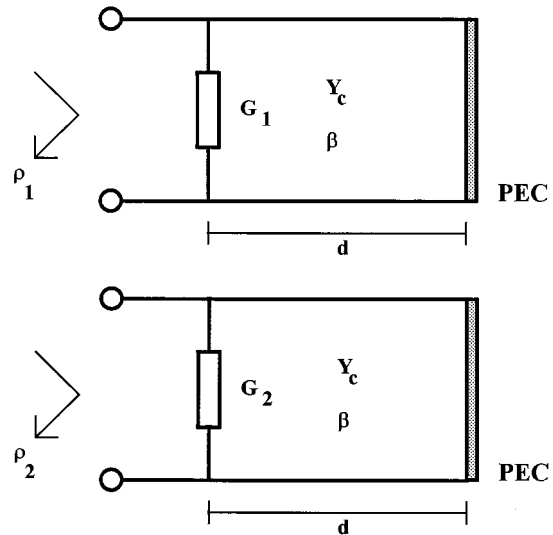
Fig. 1. Short-circuited transmission line shunted by a time-varying conductance.
