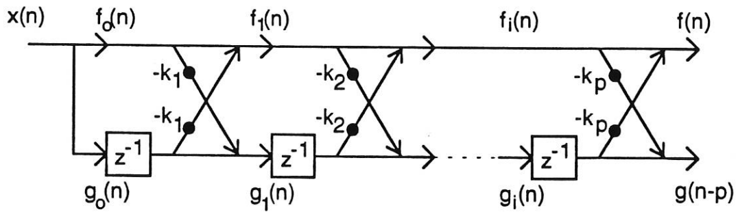
Figure 7: Lattice filter.
