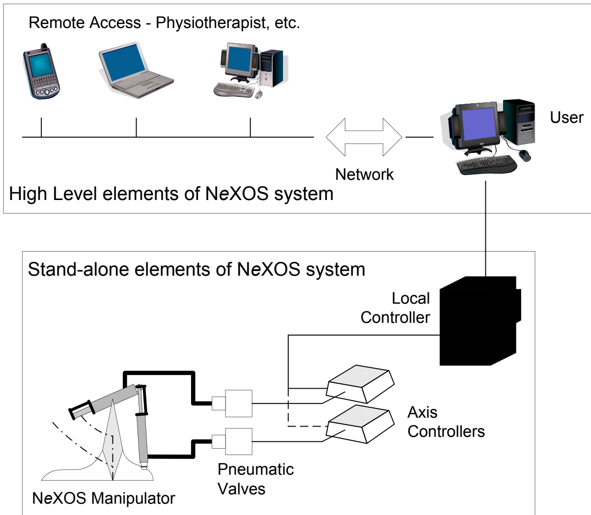
Figure 4: System configuration
