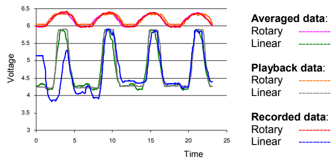
Figure 14: Comparison of averaged, recorded and playback data.
