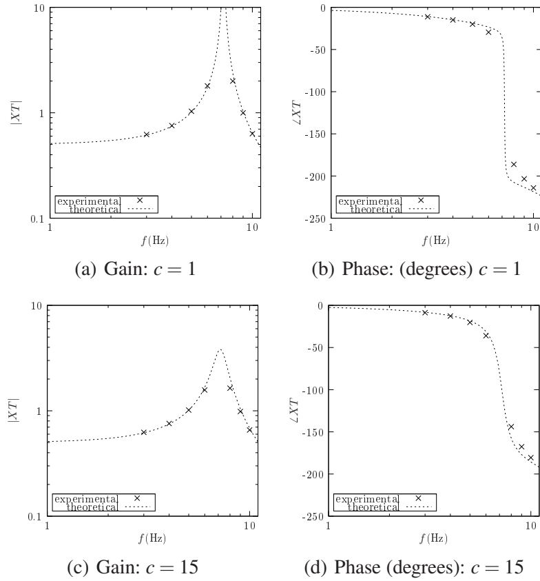
Fig. 8. Frequency response. Experimental points marked with \times are superimposed on the theoretical frequency response of T(s)X(s) (28).
