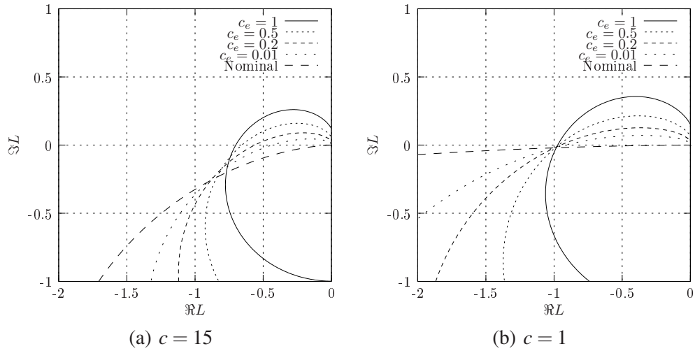
Fig. 7. Actual loop-gain. (a) L(s) (35), with damping coefficient c = 15 , is plotted for five values of damping coefficient: c_e = 1, 0.5, 0.2, 0.01 and c = 1 as well as for the nominal loop gain L_0(s) (31) of figure 4. (b) is as (a) except that the damping coefficient c = 1 ; the stability margins are smaller in this case.
