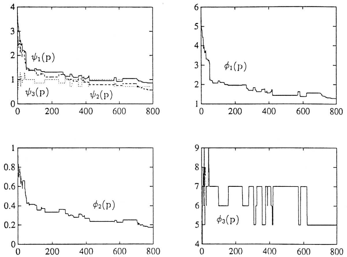
Figure 4: The convergence of the performance functions using GRBF network.
