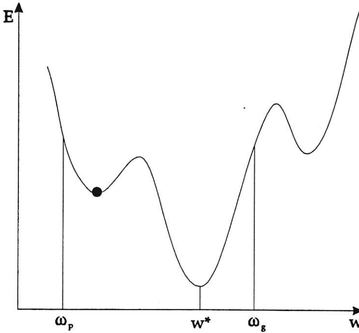
Figure 2: The objective function, E , as a function of connection strength, w — the scalar case
