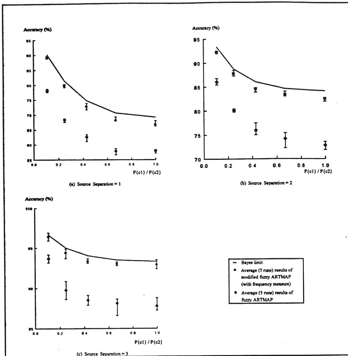
Figure 9 These graphs show the ratio of prior probabilities against the classification accuracy. All the results are bounded by the best and worst results of 5 runs.
