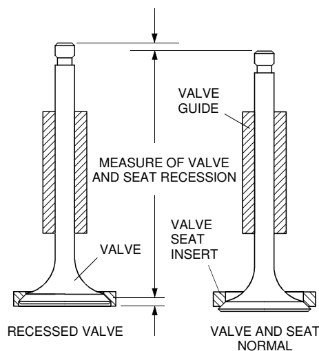
Figure 1. Valve Recession
