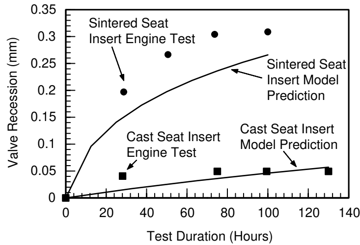
Figure 5. Model Predictions versus Engine Test Data
