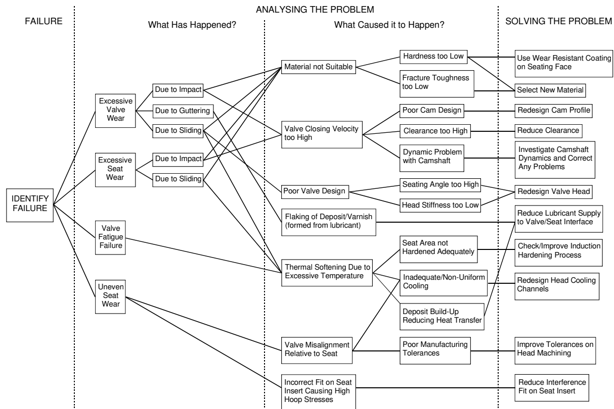
Figure 6. Solving Valve/Seat Failure Problems
