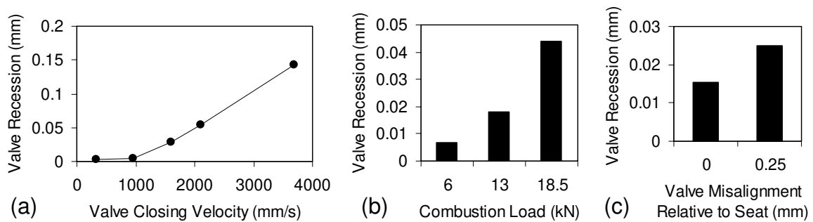
Figure 4. Valve Recession with Cast Tool Steel Seat Inserts for Increasing (a) Valve Closing Velocity (after 100 000 cycles); (b) Combustion Load (after 25000 cycles) and (c) Valve Misalignment (after 25000 cycles)
