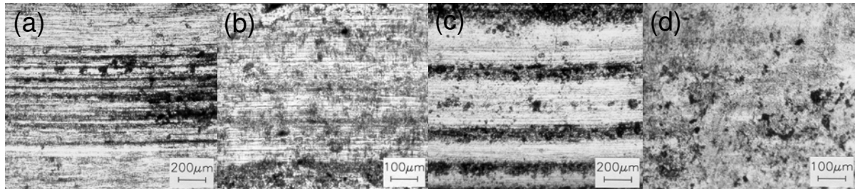
Figure 3. Laboratory Tested Valve (a) and Seat Insert (b) Compared with Engine Tested Valve (c) and Seat Insert (d)
