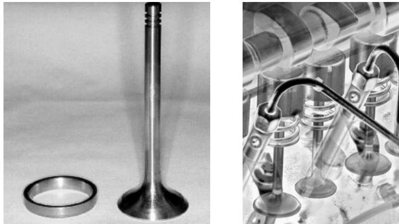
Figure 2. Valve, Seat Insert and Valve Operating System
