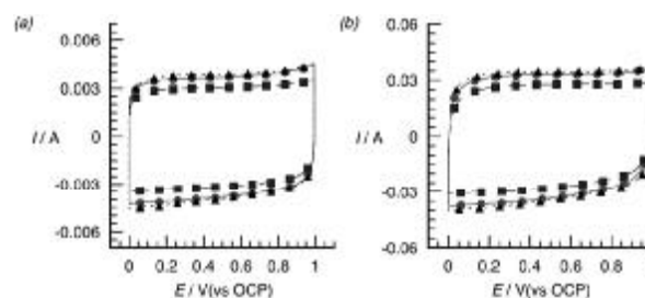
Fig. 5 Cyclic Voltammograms at (a) 10 \text{mV s}^{-1} and (b) 100 \text{mV s}^{-1} . Current is normalized based on the mass of NECM. Circles: NECM treated under hydrogen (C-H), squares: mixed hydrogen-argon atmosphere (C-HAr), triangles: argon (C-Ar).
