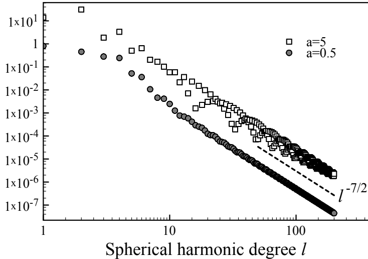
Figure 3: The spectrum E(l) of f_3 which has a nonlinear line singularity of order p = 5/2 on the intersection of the surface 1/2 + ay - z^3 = 0 with the unit spherical surface centred at the origin, for a = 1/2 and a = 5 . The dashed line confirms that, for both choices of a , the envelope scales as l^{-7/2} .
