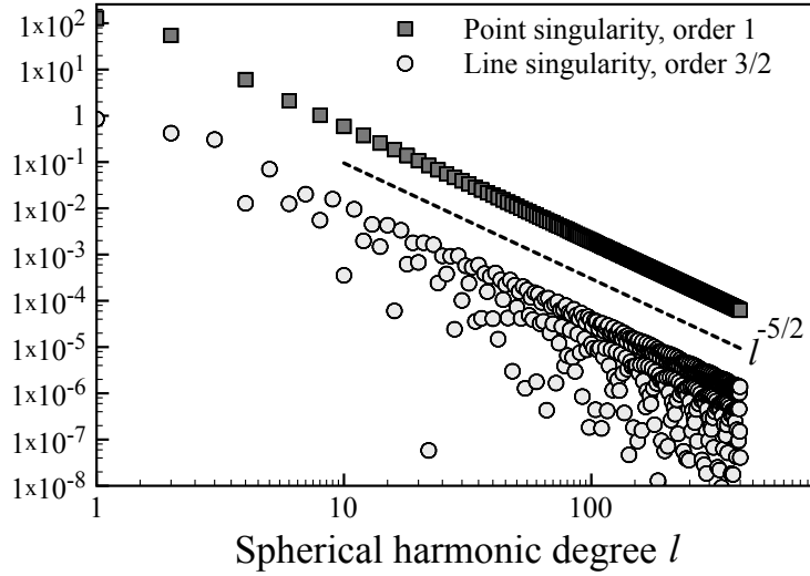
Figure 1: A comparison of the spherical harmonic spectra E(l) of a point singularity of order 1 and a line singularity of order 3/2 as defined in the text; in both cases E(l) \sim l^{-5/2} .
