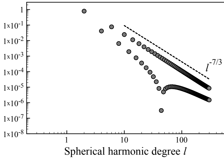
Figure 2: The energy spectrum E(l) of a function which has two line singularities of order p = 4/3 : on the lines of intersection between the planes z = 0 and y = 0 with the unit spherical surface centred at the origin. The dashed line confirms that the envelope scales as l^{-7/3} .
