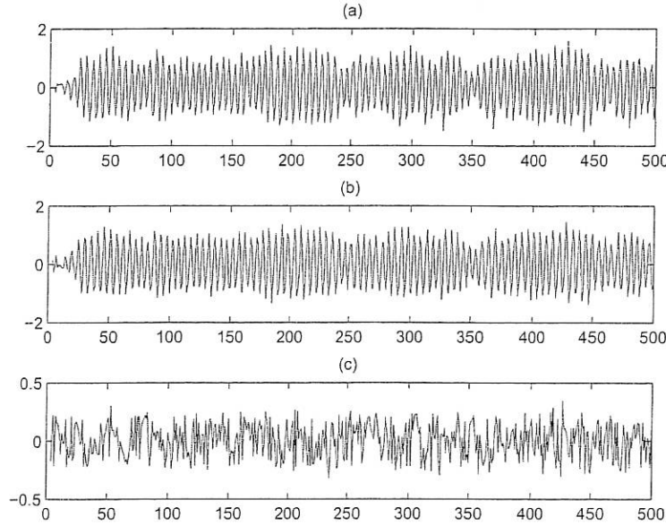
Figure 2: One-step-ahead prediction of the simulated time series in Example 1. Figure (a) indicates the system measurements, Figure (b) indicate the one-step-ahead predicted outputs for the final model with l_1 regularization and Figure (c) indicates the one-step-ahead prediction error.
