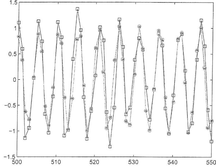
Figure 3: Many step ahead predicted output of the simulated time series in Example 1. Solid line with squares indicates the system measurements , the lines with stars and with circles indicate the model predicted outputs for the final model with l_1 and without l_1 regularization respectively.
