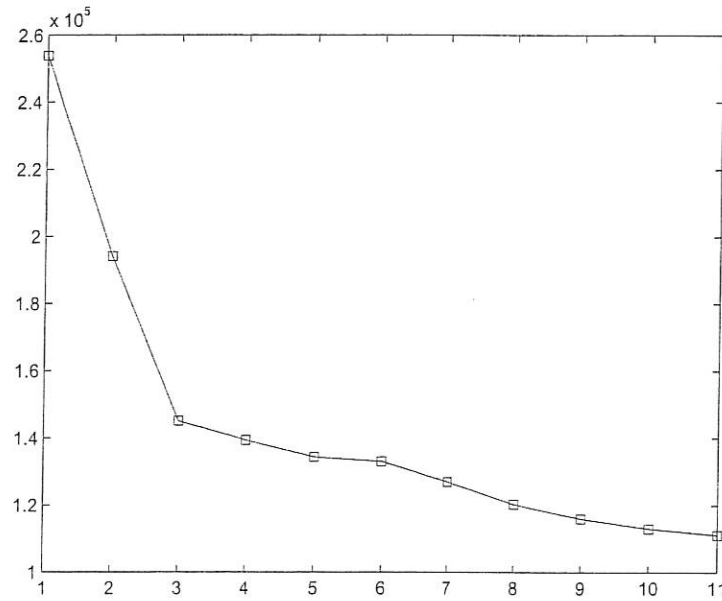
Figure 4: The estimates of the model prediction errors for different model sizes of the ozone concentration time series.
