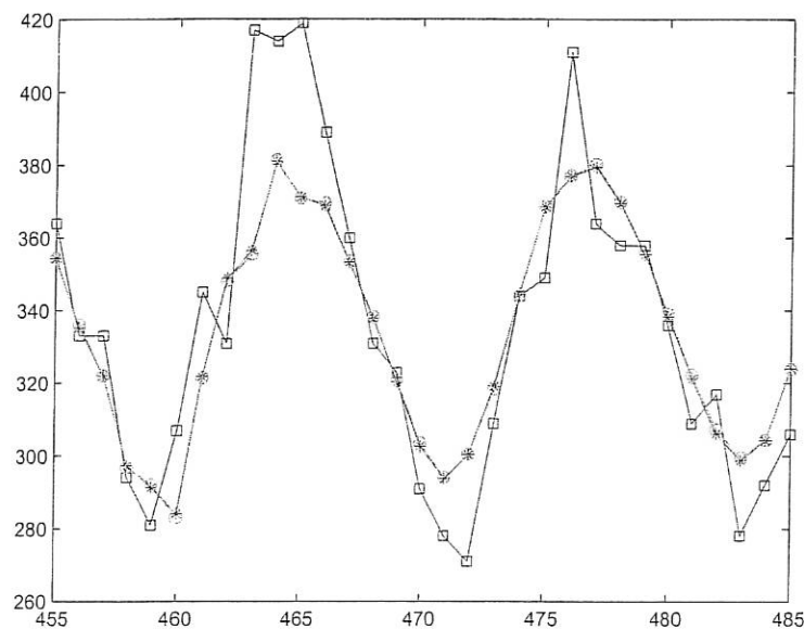
Figure 6: Many step ahead predicted output of the ozone concentration time series in Example 2. Solid line with squares indicates the ozone concentration measurements, the line with stars and the line with circles indicate the model predicted outputs for the final model with l_1 and without l_1 regularization respectively.
