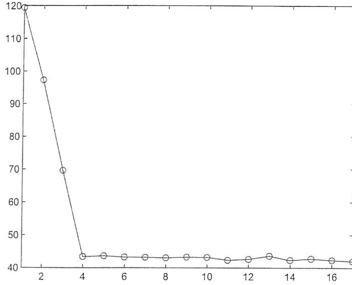
Figure 1: The estimates of the model prediction errors for different model sizes of the simulated time series.
