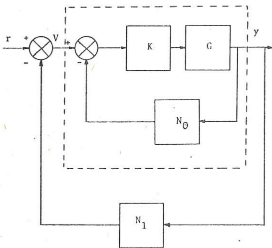
Figure 4 A system decomposition
