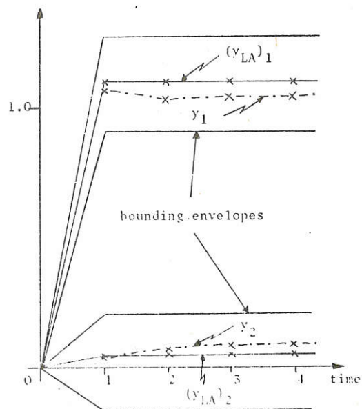
Figure 7 Closed-loop of real, nonlinear and approximate, linear feedback systems to a unit step demand in output one.
