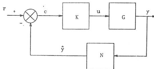
Figure 1 Nonlinear Feedback System
