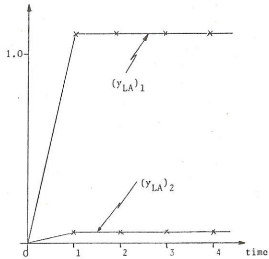
Figure 6 Response y_{LA} of approximate linear feedback system to a unit step demand in output one.
