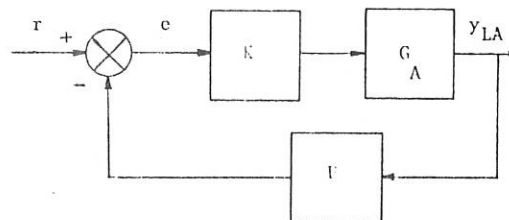
Figure 2 Linear feedback system with linear plant and measurement approximations
