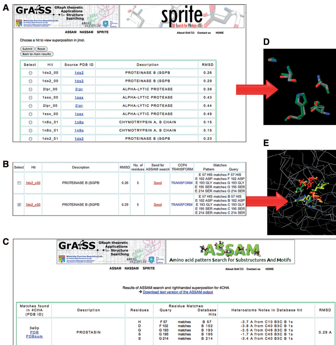
Figure 3. Snapshots of various pages from the web server showing the output of a SPRITE search using a serine proteinase structure (PDB ID: 4CHA). (A) List of motifs in the database that match to the query protein. (B) A detailed description of the results, showing the matched residues and the TRANSFORM command for CCP4; users can also opt to execute an ASSAM search on any hit of interest. (C) An example of an ASSAM search output, using the SPRITE output as a query pattern. (D) Jmol view of the superposition of a site of interest with the motif in the database that it matches to, which can be selected from page (A). (E) Jmol view showing the position of a site of interest relative to the query structure, which can be chosen from the page depicted in (B).
