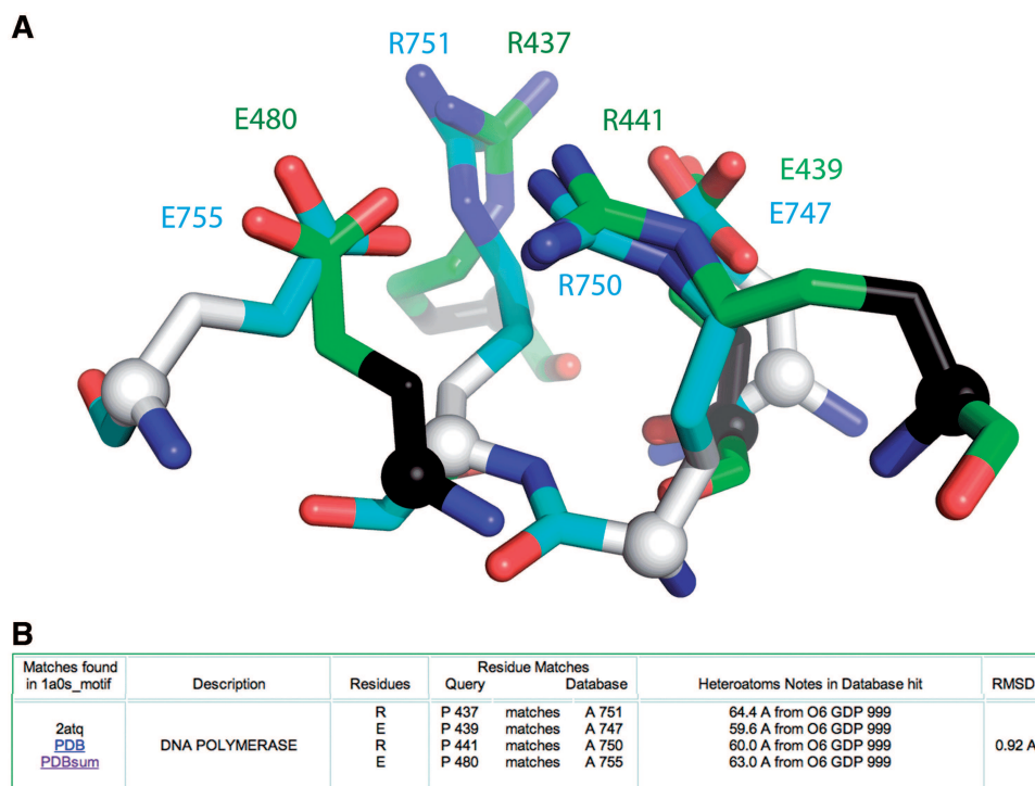
Figure 4. (A) ASSAM-derived overlap of the RERE side chain pattern from DNA polymerase (PDB ID: 2ATQ, cyan side chain carbon atoms, white C \alpha and C \beta atoms) on the search pattern from S. typhimurium sucrose specific porin (PDB ID: 1A0S, green side chain carbon atoms, black C \alpha and C \beta atoms). The C \alpha atoms are shown as spheres to emphasize the dissimilarities in the main chain positions that nevertheless permit a similar constellation of side chains. (B) Details of the hit from the ASSAM web server output.
