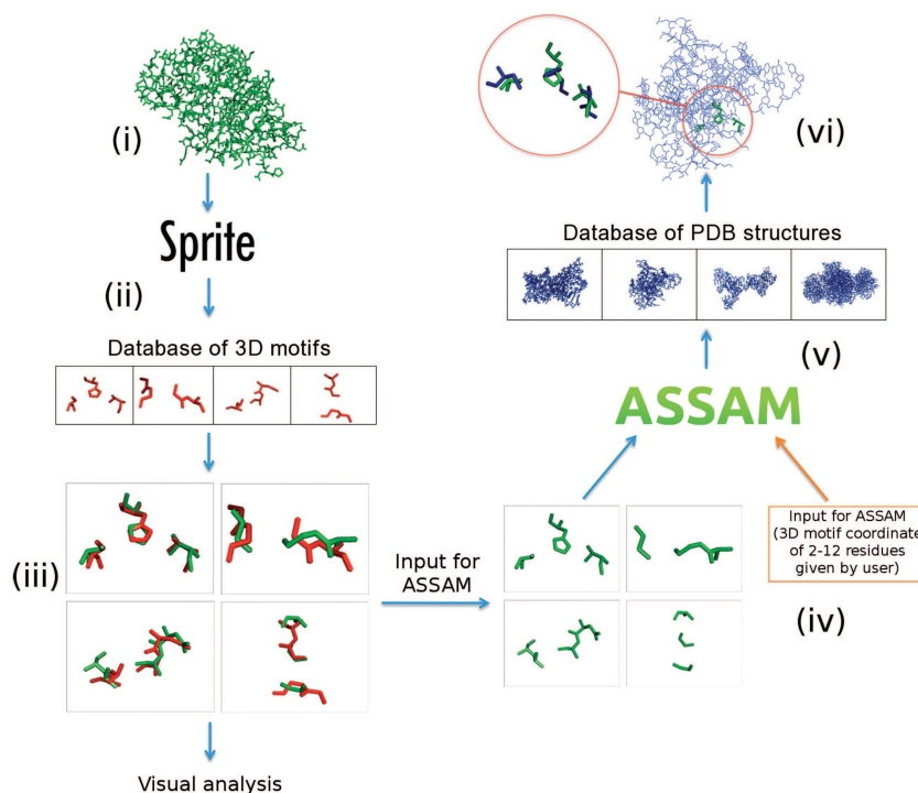
Figure 2. Diagram showing the input and output structure of SPRITE and ASSAM. (i) SPRITE accepts a whole structure in PDB format as input and (ii) compares it against a database of 3D motifs. (iii) The output is a list of amino acids in the query structure that matches to patterns in the database. (iv) ASSAM's inputs can be either any 2–12 pattern residues given by the user, or selected from the hit residues in the query structure of a SPRITE search. (v) ASSAM then compares this pattern to representative structures in the PDB. (vi) The ASSAM output is a list of PDB structures that contain the query motif. An example is shown with the superposed hit residues identified and magnified as red circles.
