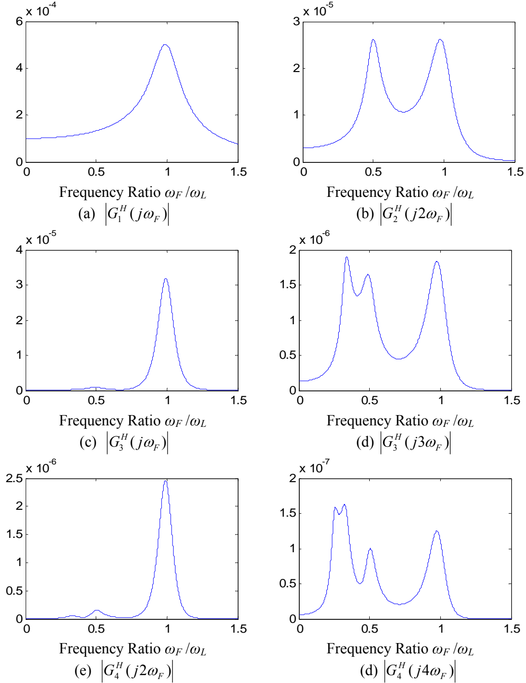
Figure 5. The NOFRFs of a nonlinear system with a 4 th order polynomial type stiffness under a harmonic loading
