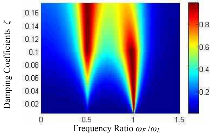
Figure 10 |G_2^H(j2\omega_F)| at different damping coefficients
