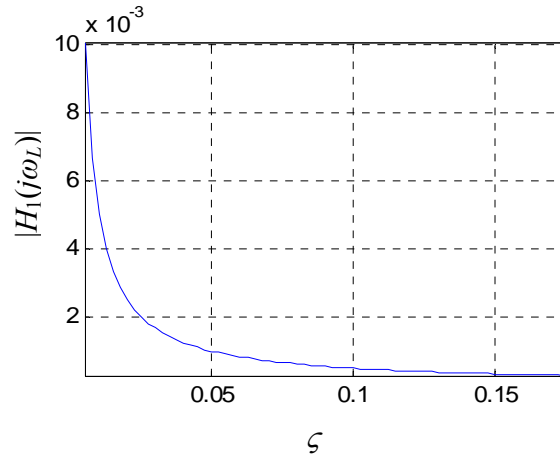
Figure 7 The dependence of a FRF at the resonant frequency \omega_L on the damping coefficient \zeta
