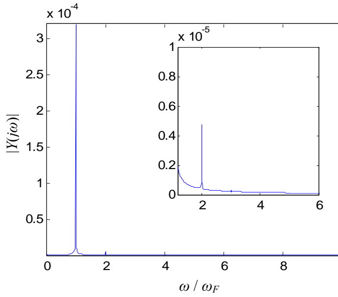
Figure 17 Output spectrum ( \zeta = 0.15 , and \omega_F = \omega_L )
