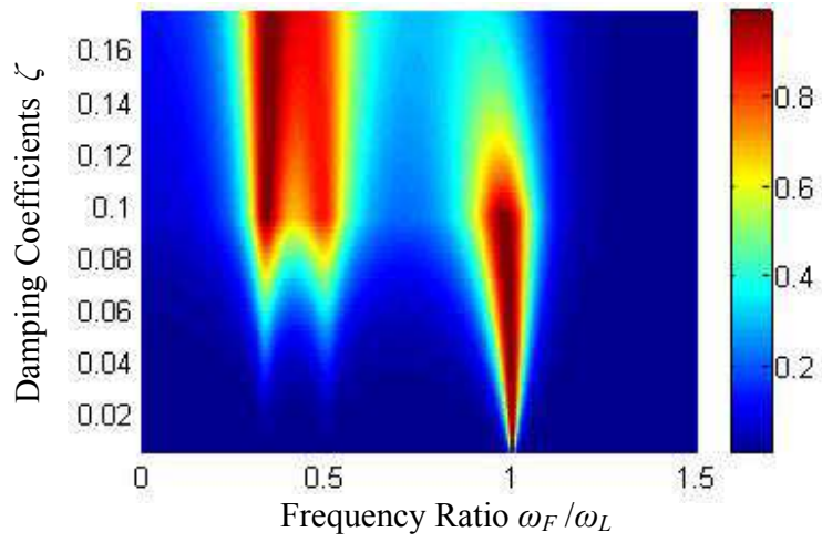
Figure 12 \left| G_3^H(j3\omega_F) \right| at different damping coefficients
