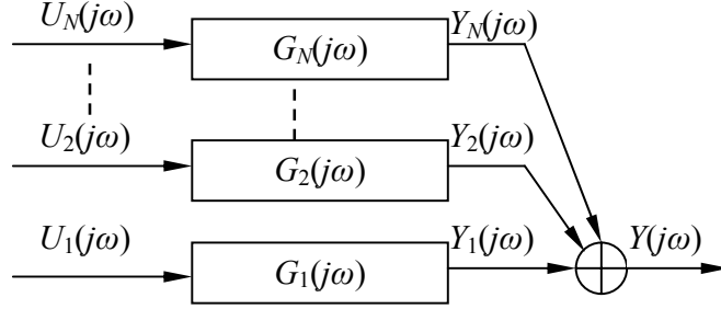
Figure 4. The output frequency response of a nonlinear system
