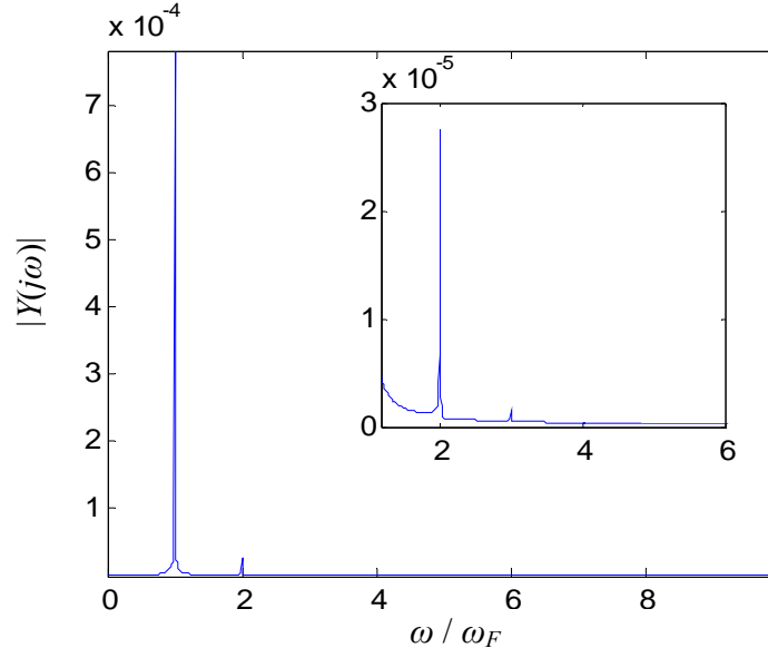
Figure 15 Output spectrum ( \zeta = 0.06 , and \omega_F = \omega_L )
