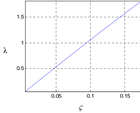
Figure 8 The dependence of \lambda on damping coefficient \zeta
