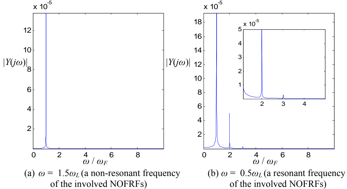
Figure 6 An illustration of the physical implication of the resonant frequencies of NOFRFs
