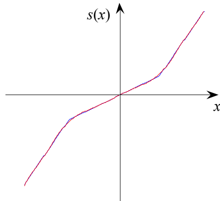
Figure 2. A polynomial approximation of a piecewise linear restoring force
