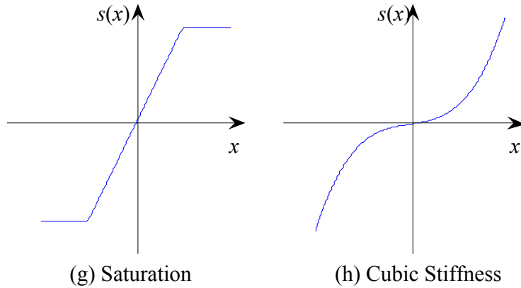
Fig 1 Most commonly used representations of nonlinear restoring force
