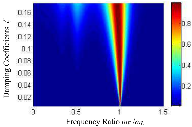
Figure 13 \left| G_4^H(j2\omega_F) \right| at different damping coefficients
