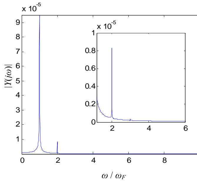
Figure 18 Output spectrum ( \zeta = 0.15 , and \omega = \omega_L/2 )
