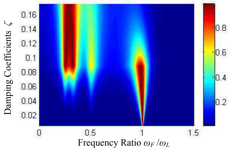
Figure 14 \left| G_4^H(j4\omega_F) \right| at different damping coefficients
