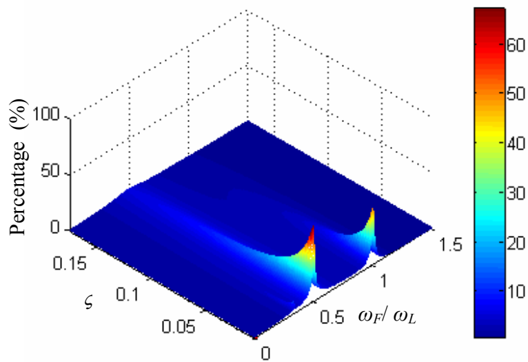
Figure 19 The percentage of the whole energy that the superharmonic components contain at different driving frequencies and different damping coefficients
