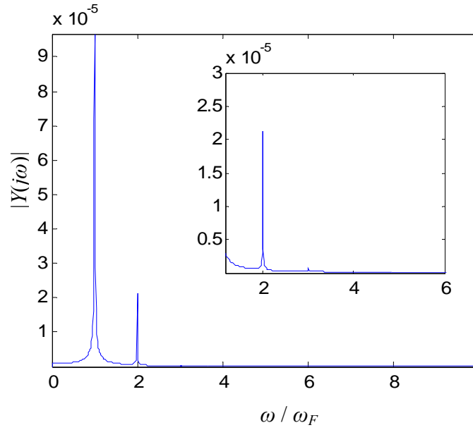
Figure 16 Output spectrum ( \zeta = 0.06 , and \omega_F = 1/2 \omega_L )
