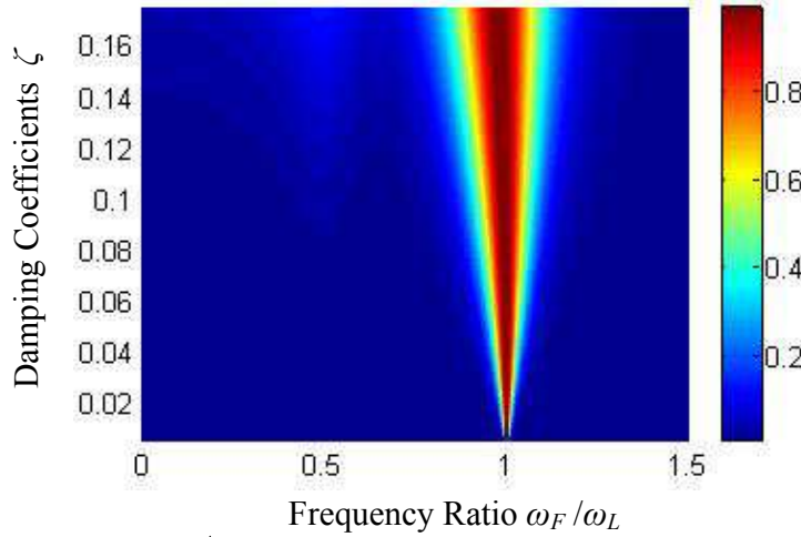
Figure 11 |G_3^H(j\omega_F)| at different damping coefficients
