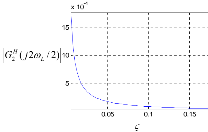
Figure 9 The dependence of \left|G_2^H(j2\omega_L/2)\right| on damping coefficient \zeta when \omega_L = 100 rad/s
