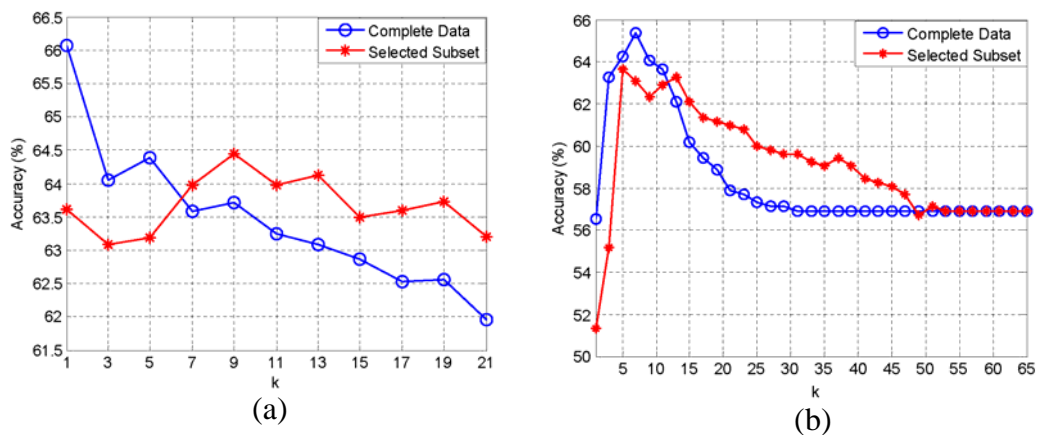
Fig. 2. A comparison of the classification accuracy based on the complete data and the associated subset, using the k -NN algorithm with different values of k . (a) for the Forest data; (b) for the Arrhythmia data.
