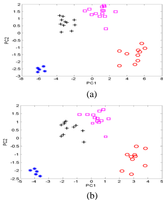
Fig. 1 Alate Adelges data plotted against the first two principal components. (a) computed from all the 19 variables; (b) computed from the first 9 selected variables listed in Table 1.
