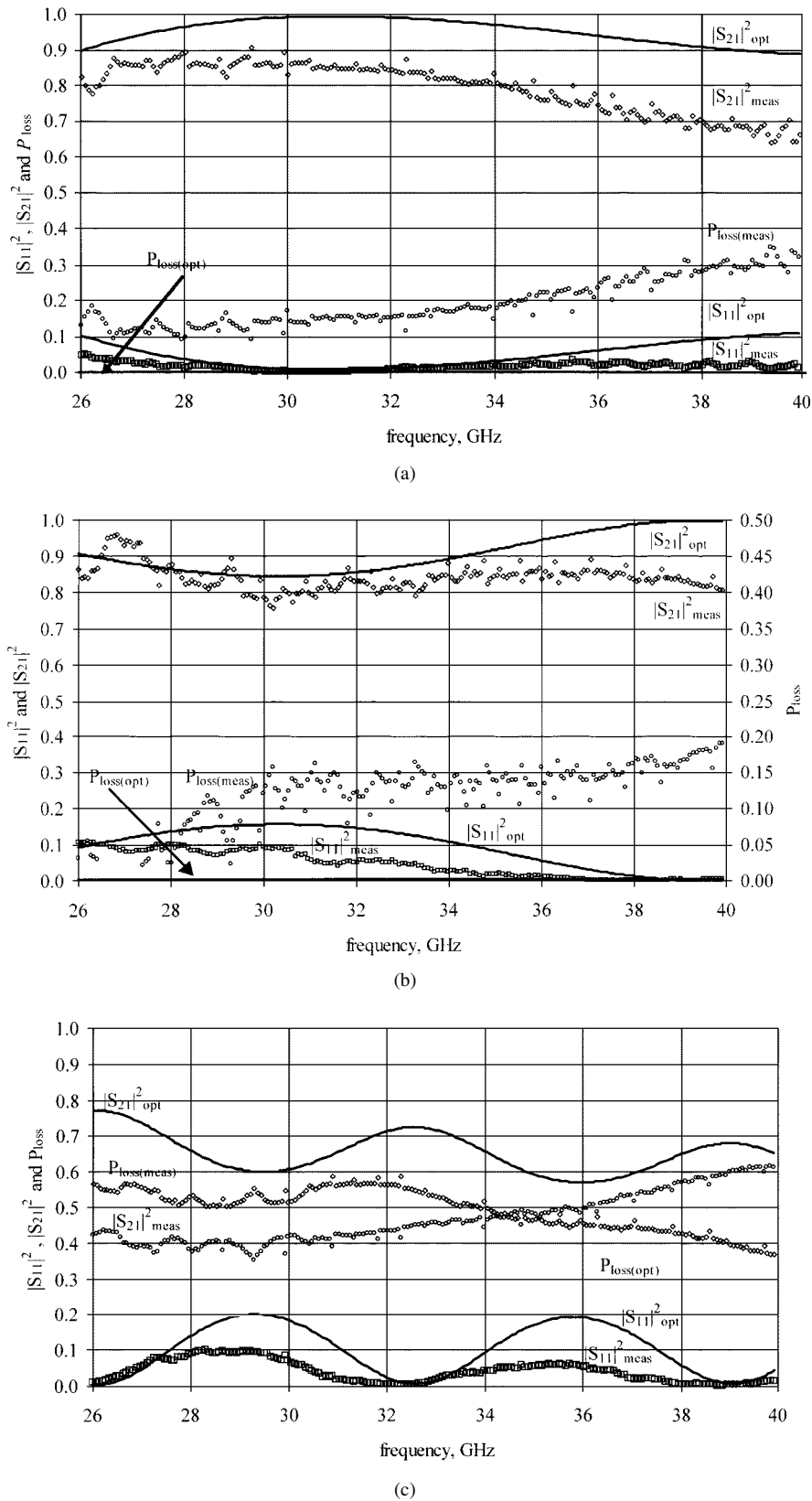
Fig. 6. Comparison between measured and predicted values of |S_{11}|^2 , |S_{21}|^2 , and P_{\text{loss}} for (a) PTFE, (b) polystyrene, and (c) nylon.
