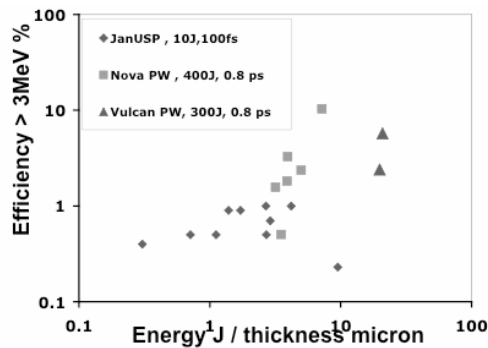
Figure 10. Collected data on conversion efficiency to >3 MeV protons versus laser energy/target thickness.
