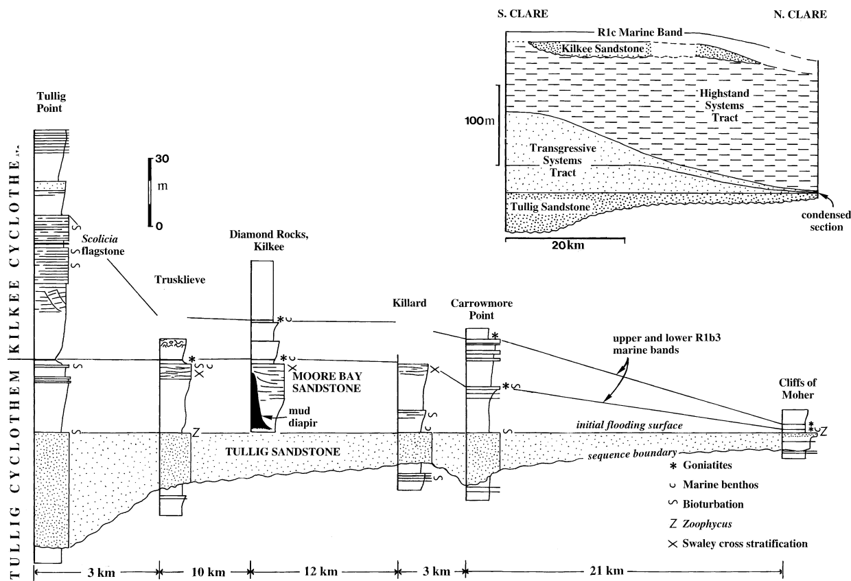
Fig. 13. Correlation of the Tullig to Kilkee Cyclothem transition in County Clare showing the rapid southward thickening of strata between the initial flooding surface that caps the Tullig Sandstone and the upper R1b3 Marine Band. The inset figure shows the thickness variations of the interval between the base of the Tullig Sandstone and the top of the Kilkee Cyclothem. This reveals the retrogradational nature of the strata in the main figure and the subsequent progradation of the higher levels of the Kilkee Cyclothem which are consequently interpreted to be a transgressive and highstand systems tract, respectively.
