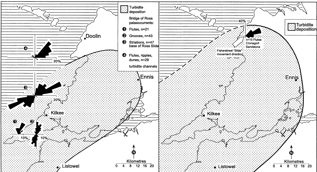
Fig. 7. Evolving palaeogeography of the WINB from earliest Alportian to mid Kinderscoutian times showing north-eastwards progradation of Ross Formation turbidites. Palaeocurrent vectors from the turbidites and interpreted movement directions of slumps consistently indicate a downslope direction to the north-east.
