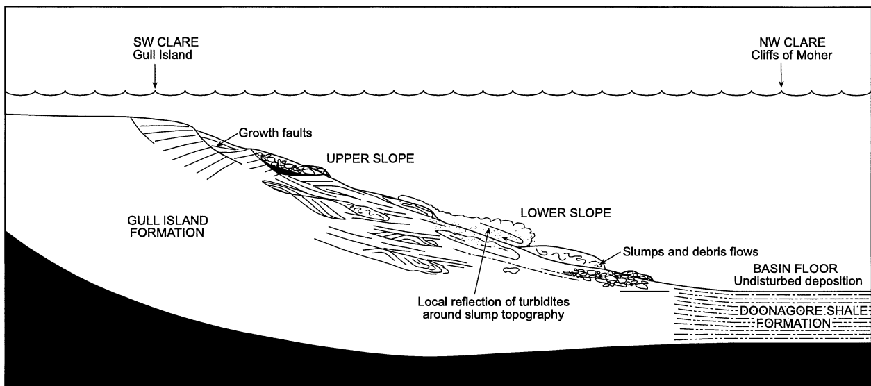
Fig. 10. Depositional model for the Gull Island Formation. The lower slope is dominated by slumps and turbidites whilst up-slope growth faults become the dominant style of deformation (cf. Rider, 1978). Note that the vertical scale is much exaggerated for clarity.
