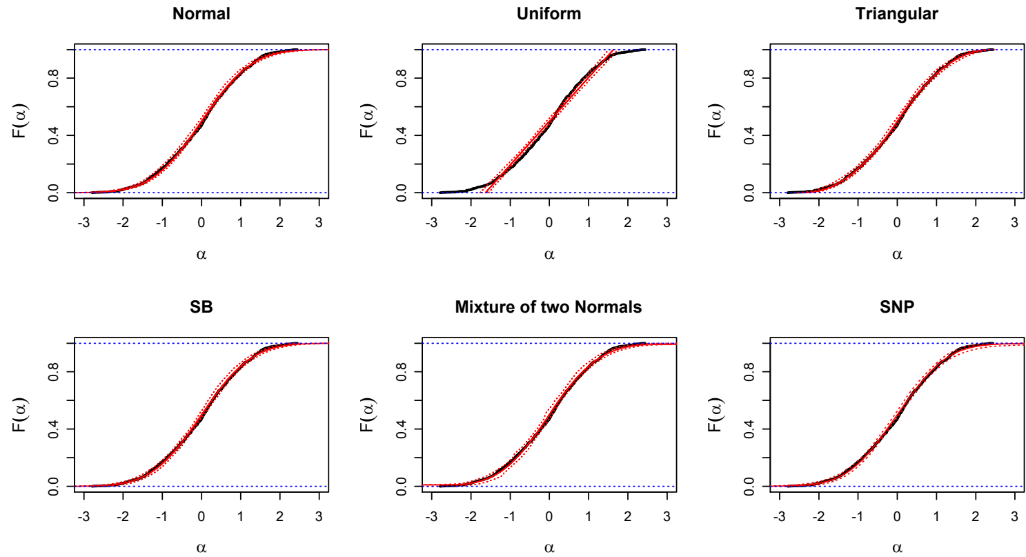
Figure 6: CDF plots for \alpha in models estimated on N data
