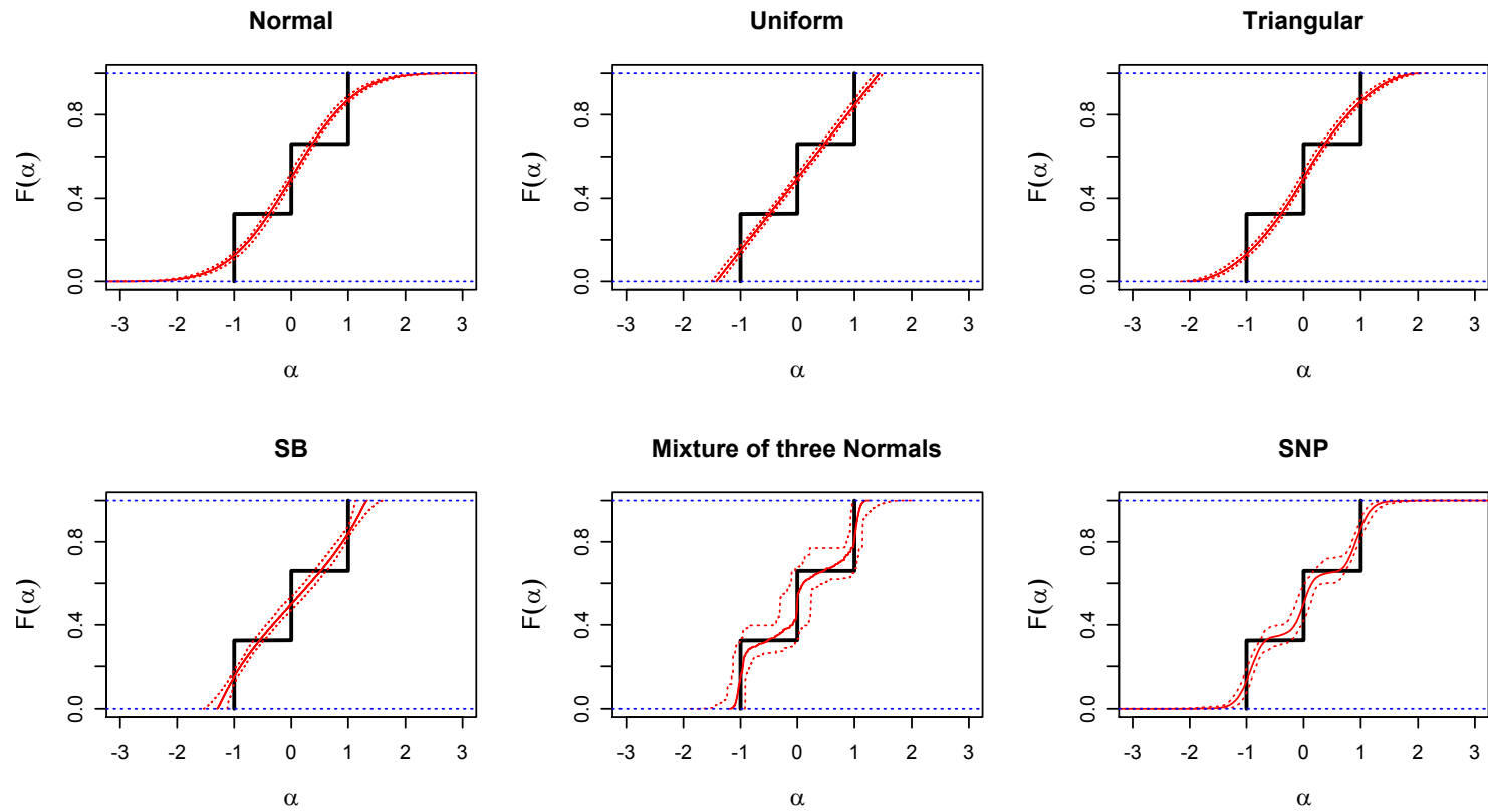
Figure 4: CDF plots for \alpha in models estimated on DM(3) data
