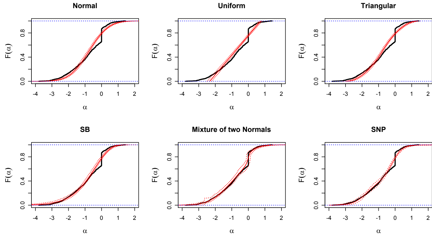
Figure 7: CDF plots for \alpha in models estimated on NM data
