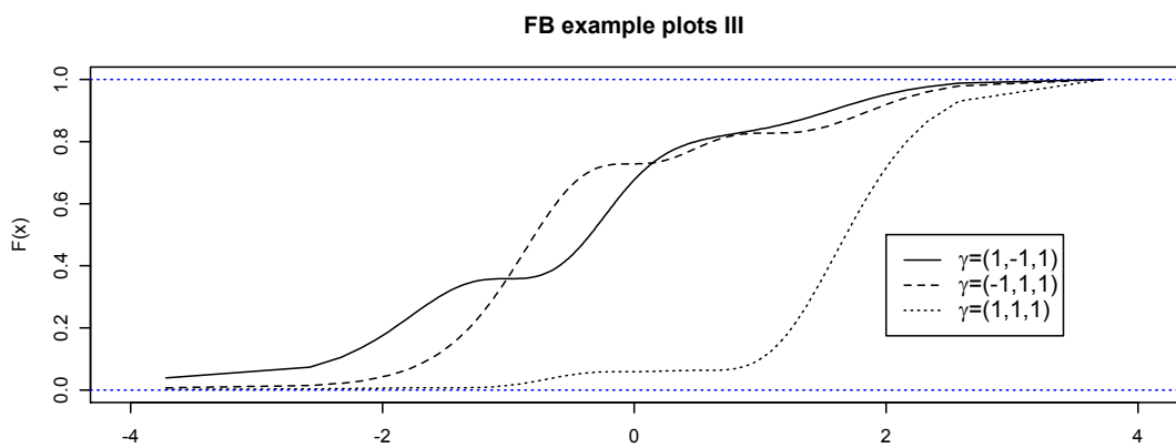
Figure 1: CDF plots for various FB distributions
