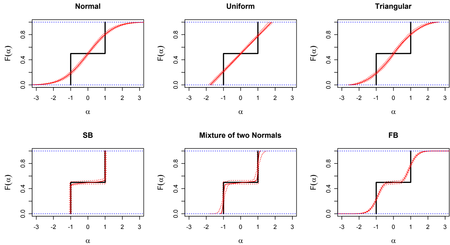
Figure 3: CDF plots for \alpha in models estimated on DM(2) data
