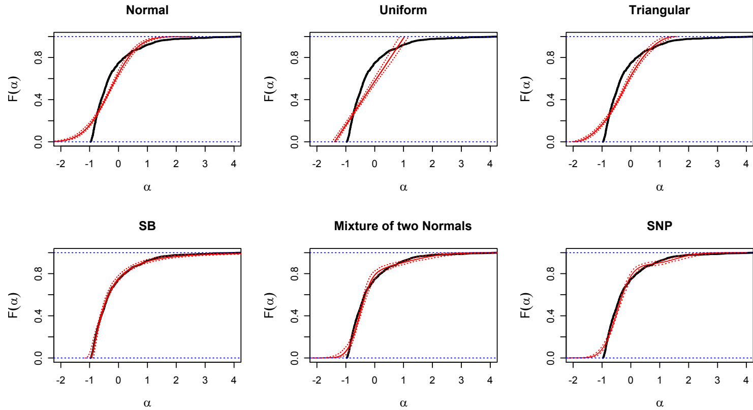
Figure 5: CDF plots for \alpha in models estimated on LN data
