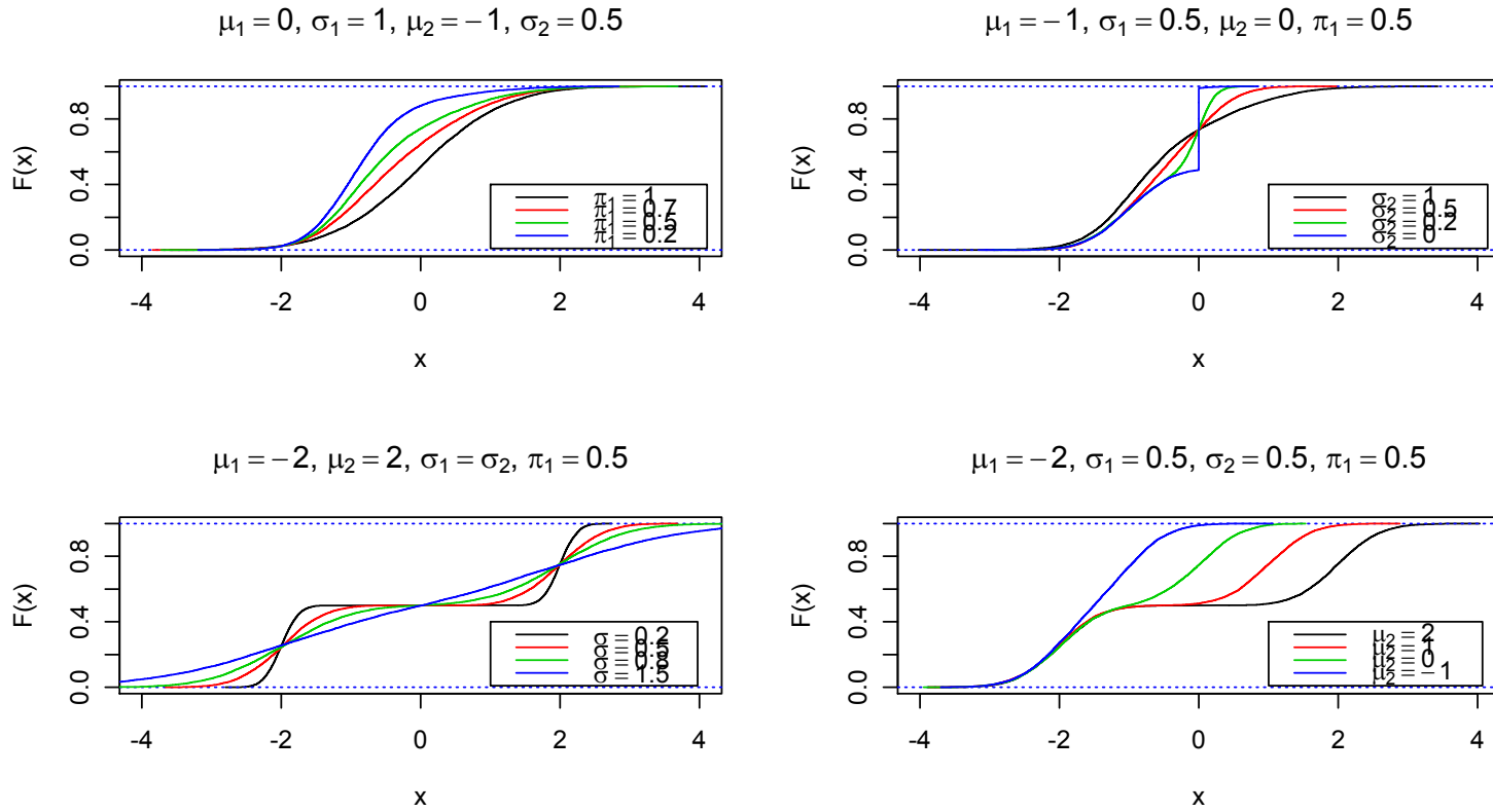
Figure 2: CDF plots for various mixtures of two Normal distributions
