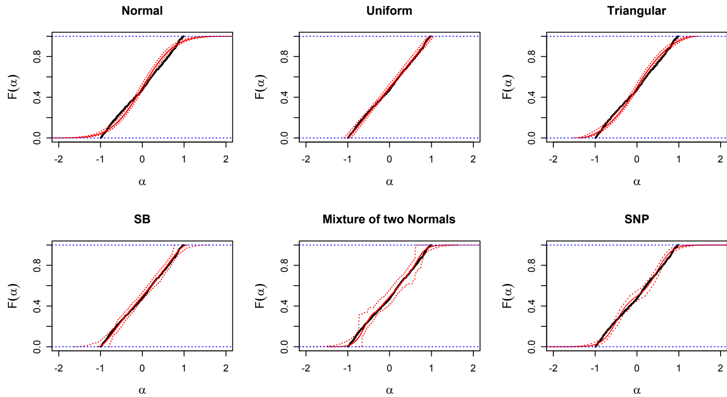
Figure 9: CDF plots for \alpha in models estimated on U data
