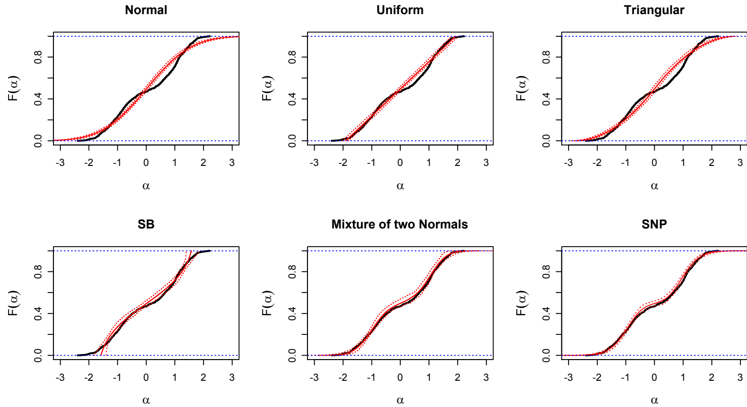
Figure 8: CDF plots for \alpha in models estimated on 2N data
