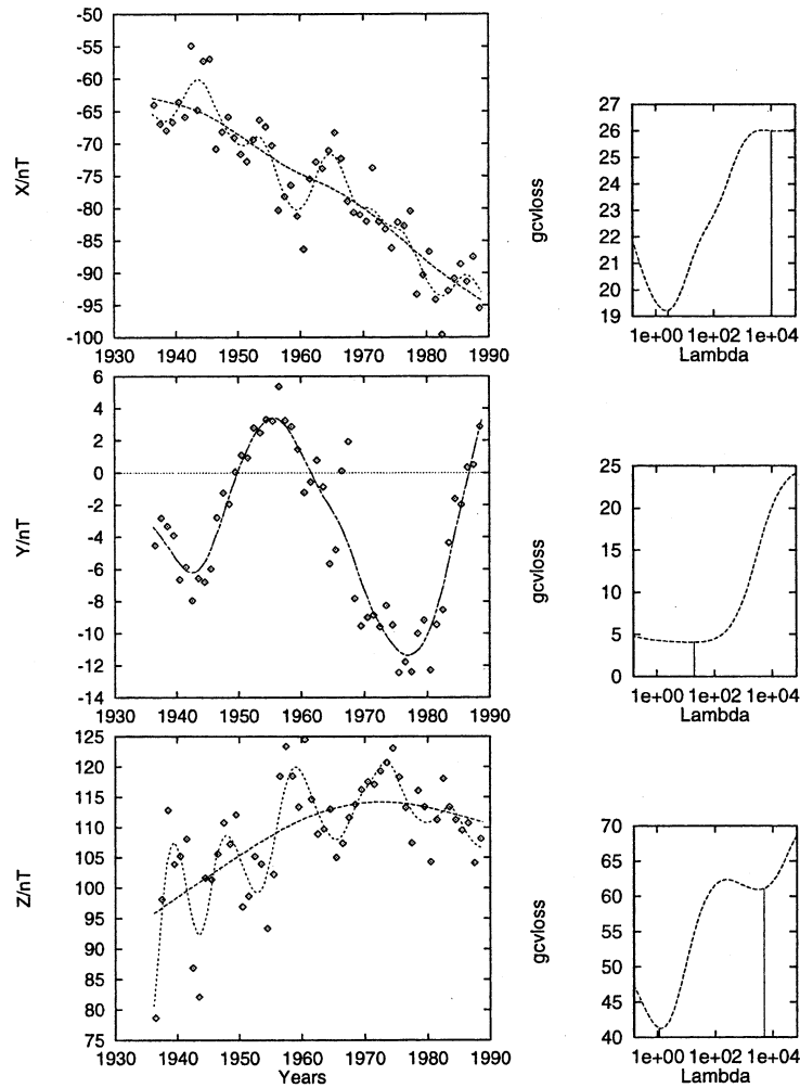
Figure 1. Champon-la-Forêt: the left-hand figures show the crustal correction in the three components X , Y and Z (diamonds) and for each component two smooth curves that fit the data. The smoothness of these curves is controlled by a parameter \lambda , which is estimated by cross-validation and associated with a minimum of the GCVLOSS curves shown in the figures on the right-hand side.
