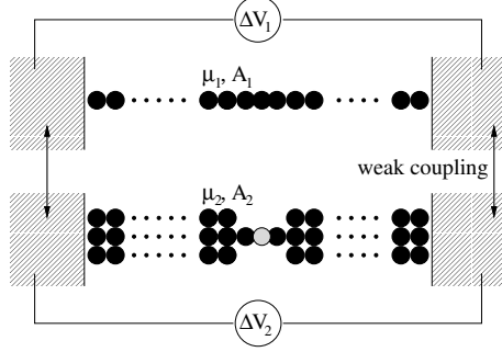
FIG. 1: Compound system 1+2 (see text) and related quantities.
