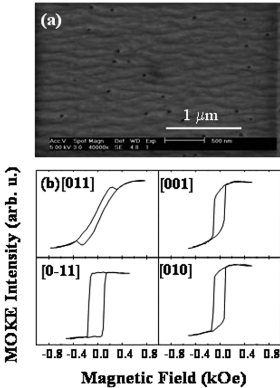
Fig. 4. (a) The SEM micrograph of magnetite nanostripes formed on GaAs(100) substrate. (b) The horizontal axis is parallel to the [011] direction MOKE loops of the Fe nanostripes obtained along four crystallographic directions for a coverage of 4.2 nm.
