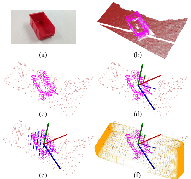
Fig. 3: Object point cloud processing, featuring the storage bin as the object in (a). Registered and segmented multi-view point cloud in (b) is then downsampled (c) and object/table coordinate frames (transformation matrices) are computed (d). The object’s bounding box is sampled in (e), and the table special ellipsoid is constructed in (f).
