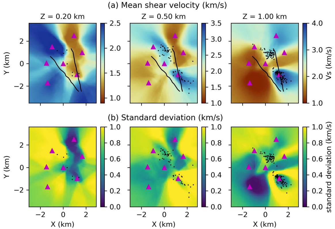
Figure 6. Horizontal slices through the 3D shear velocity model at depth of 0.2 km (left), 0.5 km (middle) and 1.0 km (right) obtained using body wave travel time data only. The upper panels (a) and the bottom panels (b) show the mean velocity maps and standard deviation maps, respectively. At each slice events within 0.2 km of the depth are plotted. Black lines show faults that appear in the study area.
