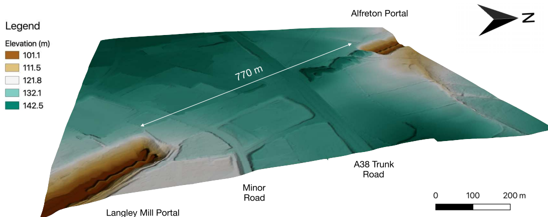
FIG. 2. Representation of the Alfreton Old and New Tunnels and surrounding using open-source LiDAR data [9].
