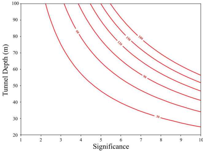
FIG. 1. Significance of an open shaft observation as a function of tunnel depth (overburden) and measurement time.
