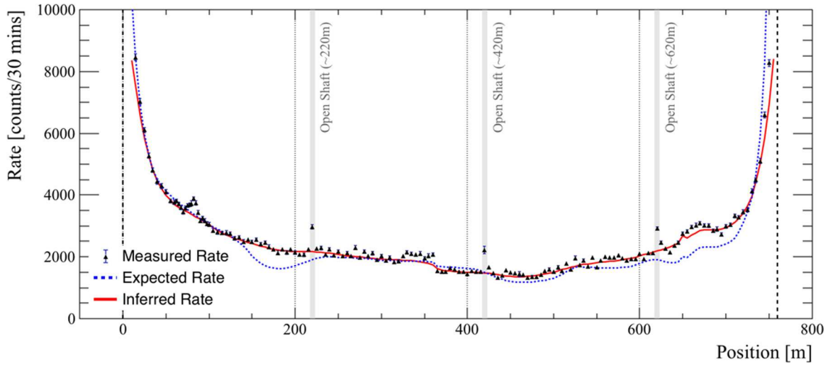
FIG. 4. Comparison of measured muon flux rate with the expected rate (from topographical information) and inferred rate along the full length of the tunnel. Distances measured from the Langley Mill entrance.
