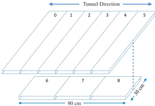
FIG. 3. Schematic of the scintillator configuration; the dotted line represents the vertical in the system.
