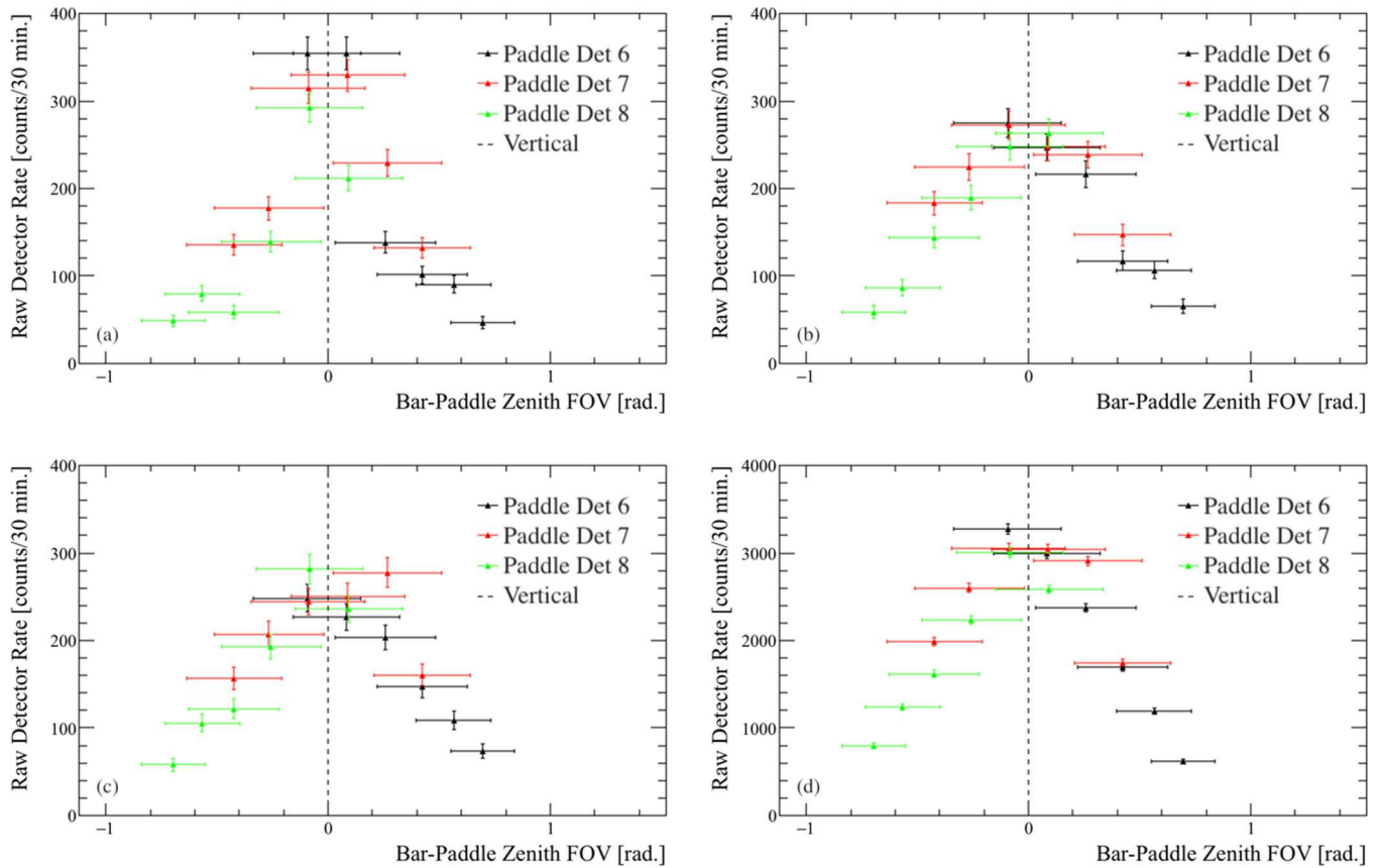
FIG. 6. Muon flux rates on upward-looking bar-paddle combinations for the following points along the tunnel: 625 m (a), 650 m (b), 700 m (c), and open sky (d) as a function of the field of view of those detector combinations.
