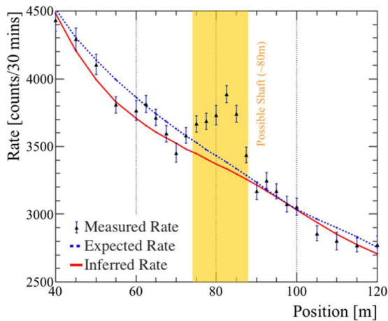
FIG. 7. Comparison of measured muon flux rate with the expected rate and inferred rate around the suspected hidden shaft at 80 m.
