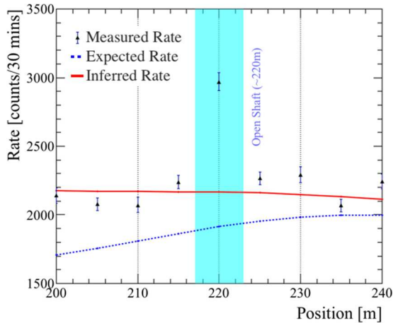
FIG. 5. Comparison of measured muon flux rate with the expected rate and inferred rate around the known open shaft at 220 m from the Langley Mill portal end of the tunnel. The inferred rate is a refined estimate using the data to update the overburden estimate as discussed below.
