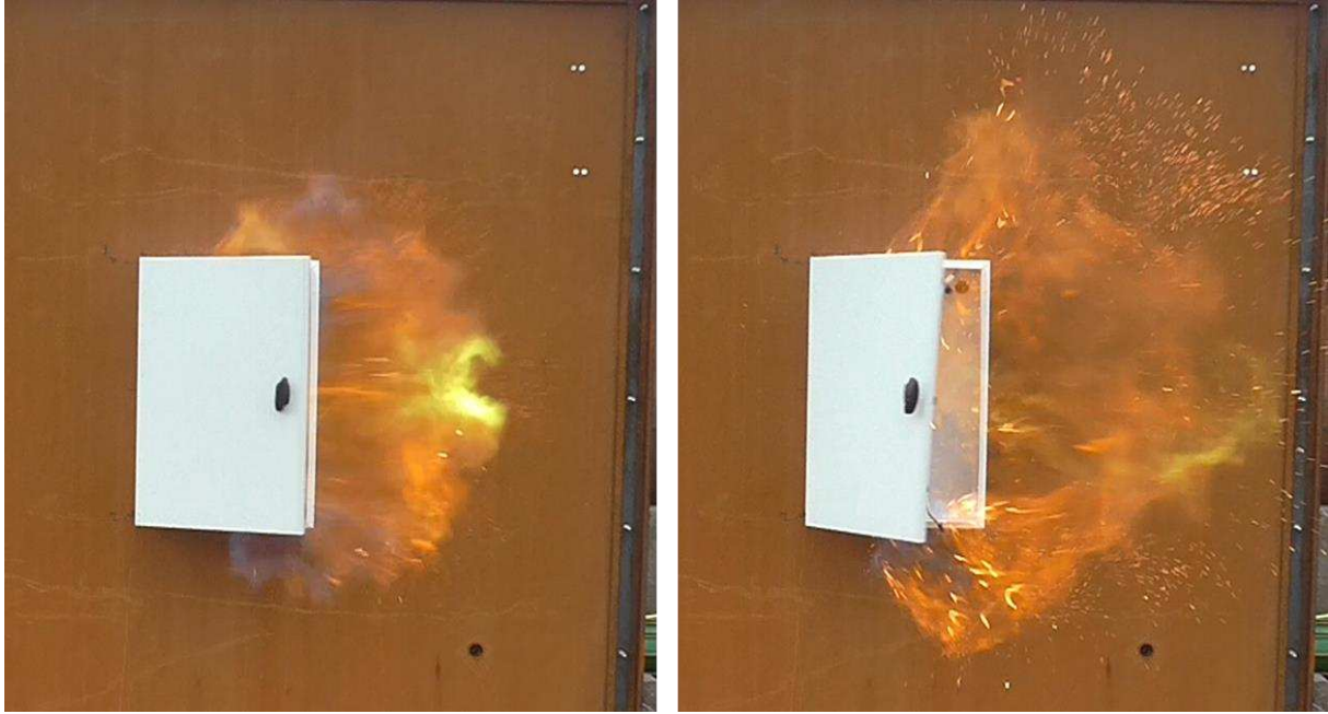
Figure 10 - front view of venting flame shape in test 3; frame interval 20 ms
