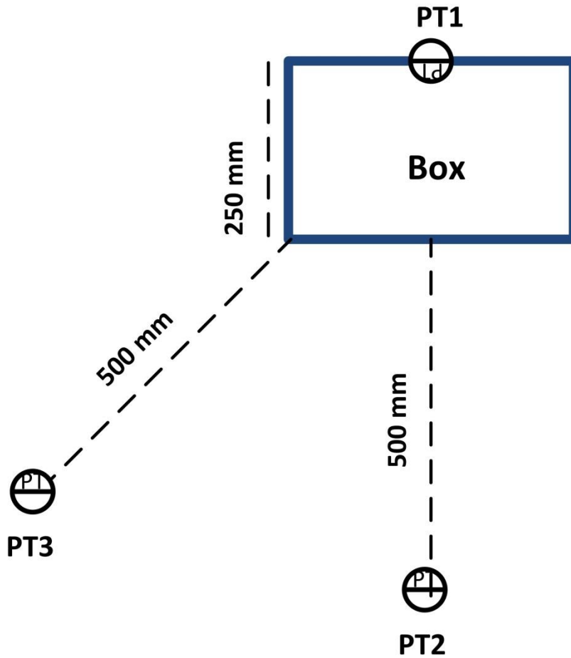
Figure 3 - Plan view of location of pressure transducers (PT)
