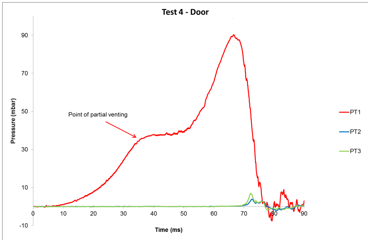
Figure 5 - Pressure trace for test 4
