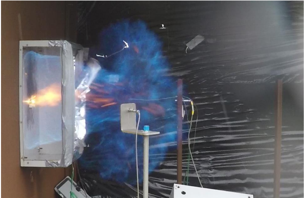
Figure 7 - Test 1 – initial mushroom flame, typical of rolling vortex bubble venting
