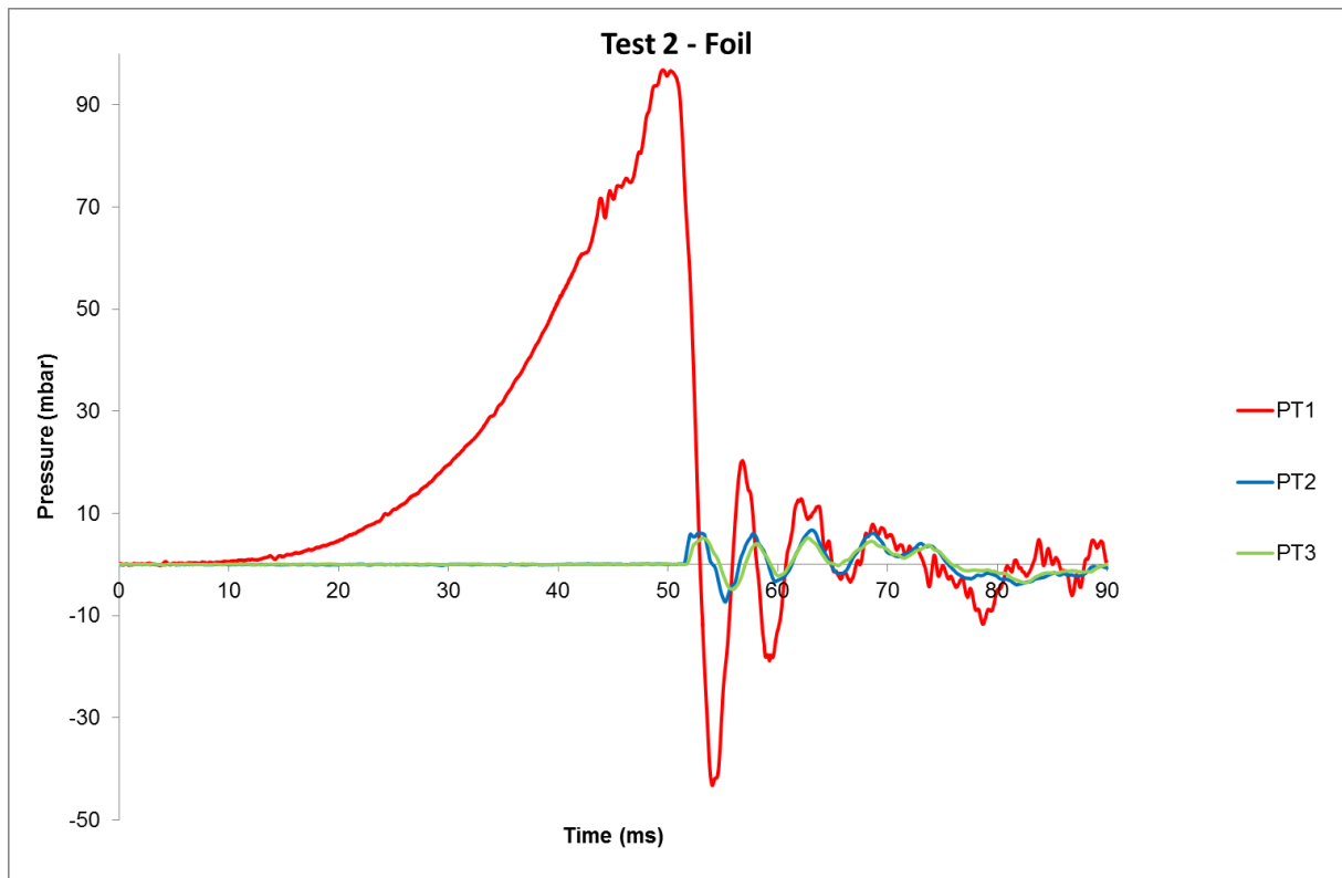
Figure 4 - Pressure trace for test 2
