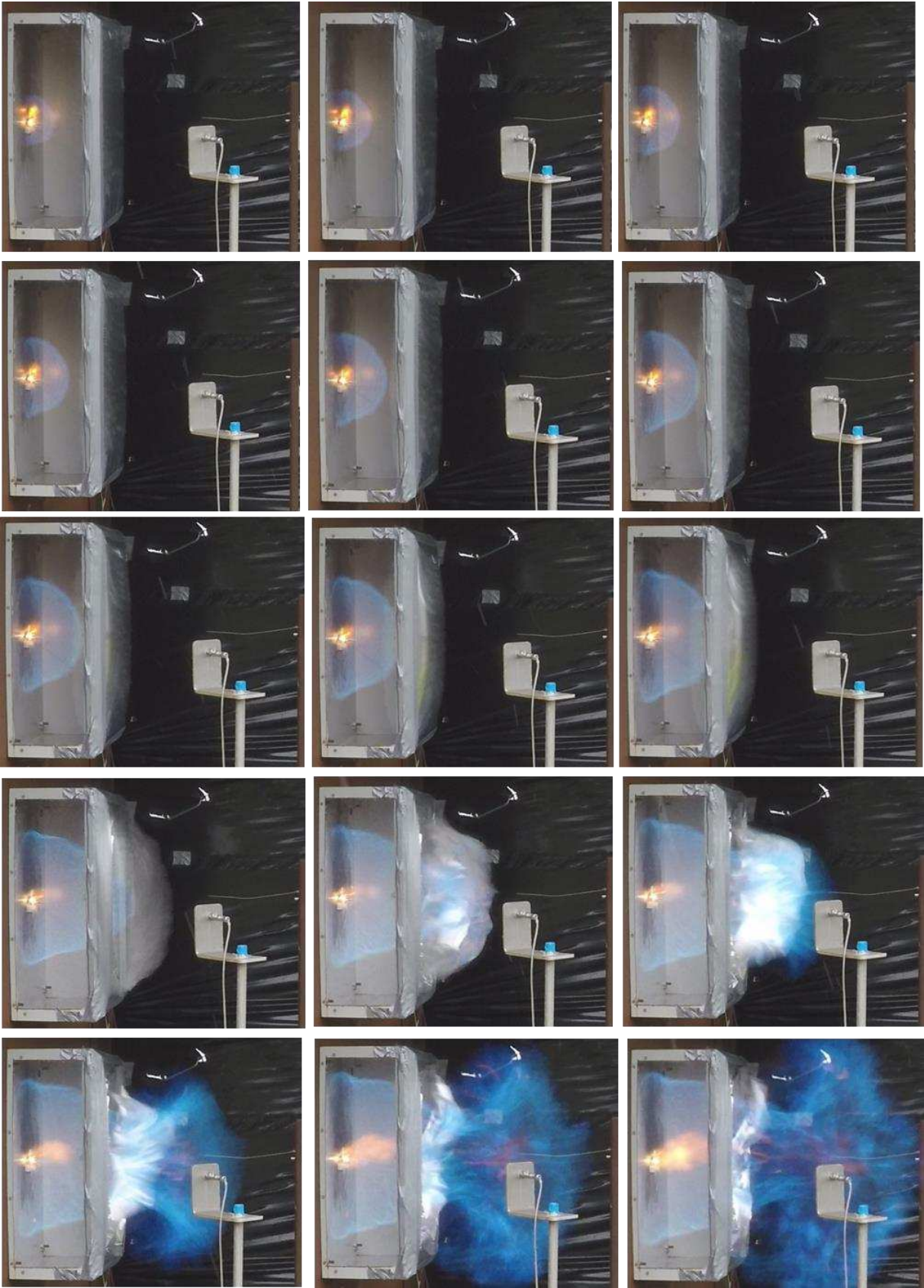
Figure 6 - flame development in test 1; frame intervals 4.17 ms
