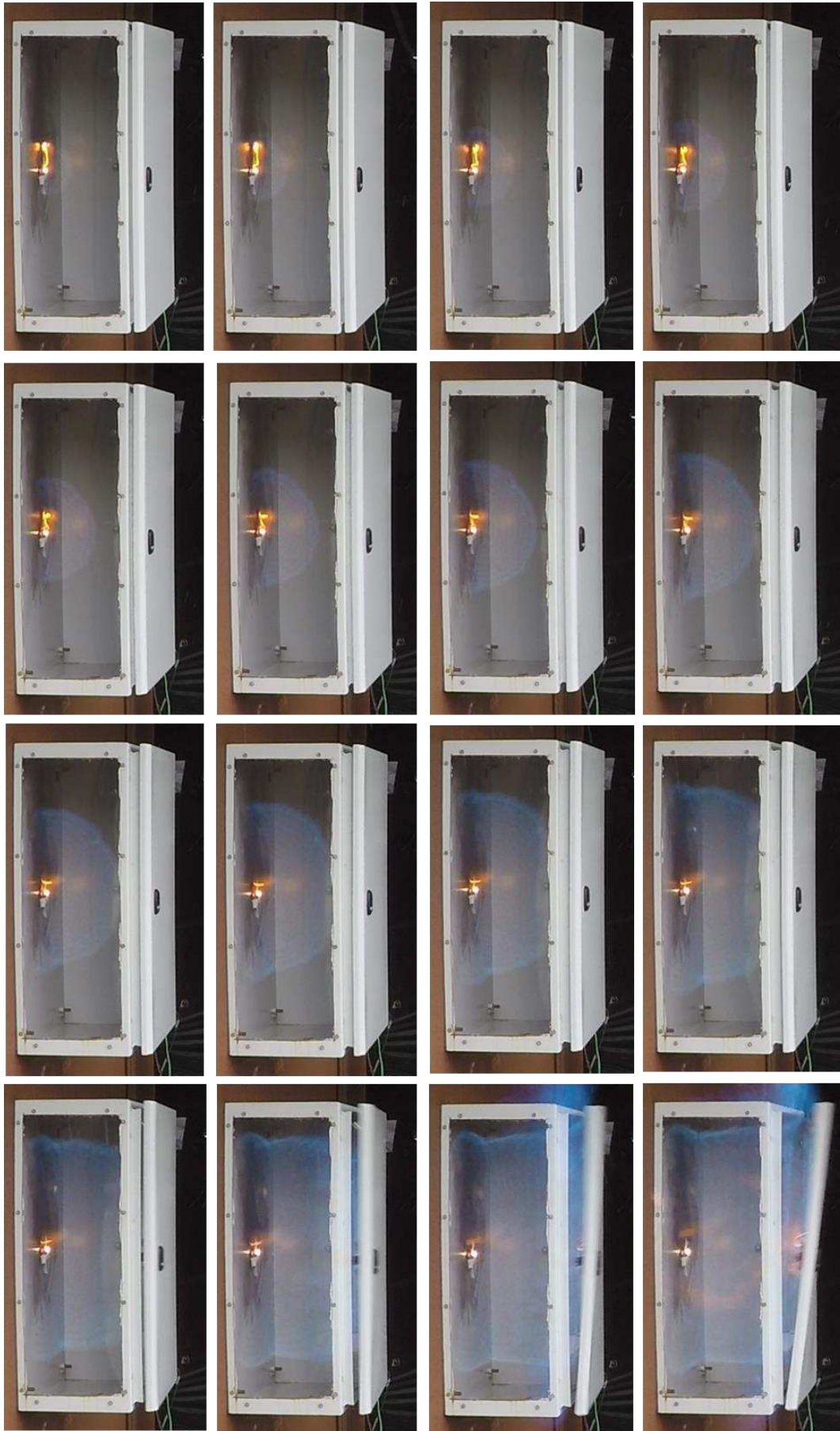
Figure 9 - Flame development in test 4; frame intervals 4.17 ms
