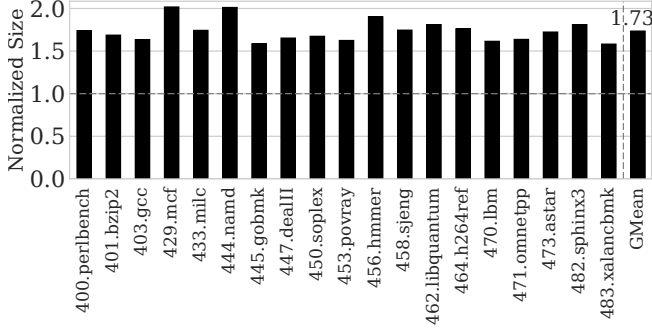
Figure 5. Average normalized function size, before and after register demotion, across all functions in each program from the SPEC 2006 benchmark suite. Register demotion increases function size by almost 75% on average.
