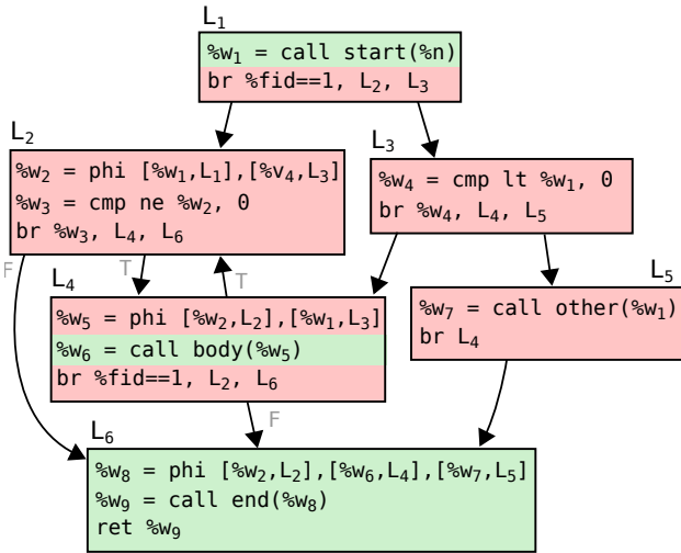
Figure 3. Desired merged function that can be produced by an expert. An extra argument called %fid is used to select between the two functions. This represents a gain of about 20% in the total number of instructions.
