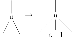
FIGURE 2. Construction of Q_{\underline{u}}^{(2)} .
