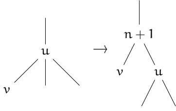
FIGURE 3. Construction of Q_u^{(3)} .
