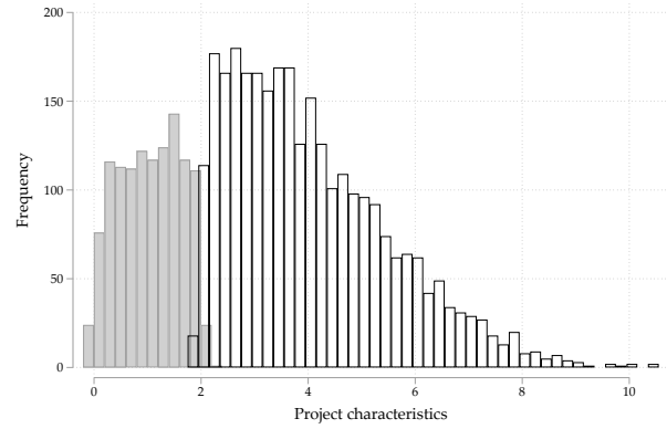
(b) Full additionality, small errors
