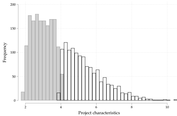
(c) Zero additionality, DFI funds > opportunities
