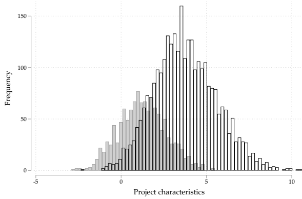
(a) Full additionality, large errors
