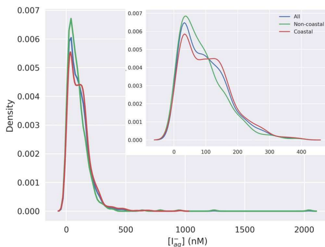
Fig. 2 Estimated probability density function (PDF; kernel density estimate) for sea surface iodide observations. Plot shows all data (blue) combined, and open ocean (green) and coastal (red) data treated separately. Expanded inset shows values < 400 nM only. Figure produced with Python Matplotlib 79 and Seaborn 80 packages.
