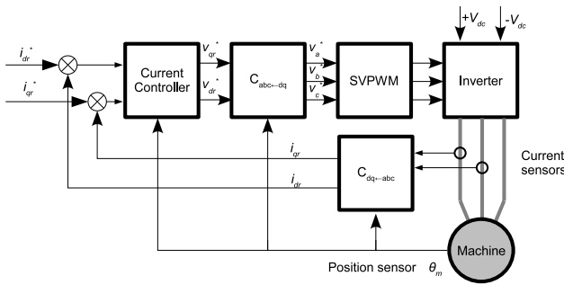
Fig. 3. Schematic of Current-Controlling Drive System
