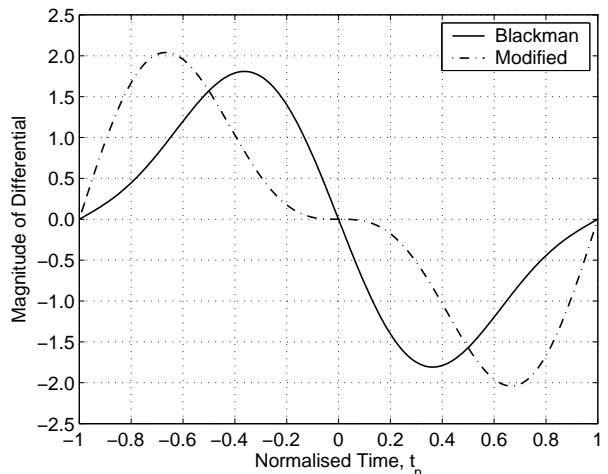
Fig. 7. Differential of Blackman-Type Windows
