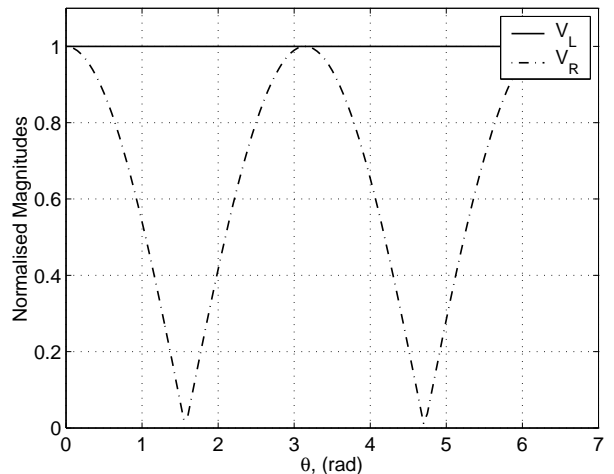
Fig. 5. Normalized Magnitudes of Injection Voltages for \theta_F = 0^\circ
