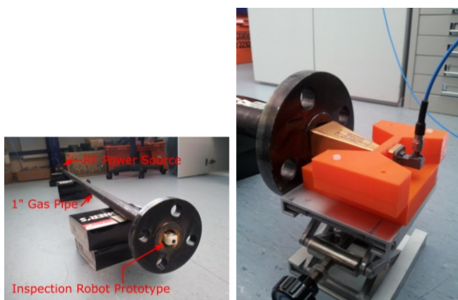
Fig. 6 Pipe measurement setup, including method of supplying RF power.
