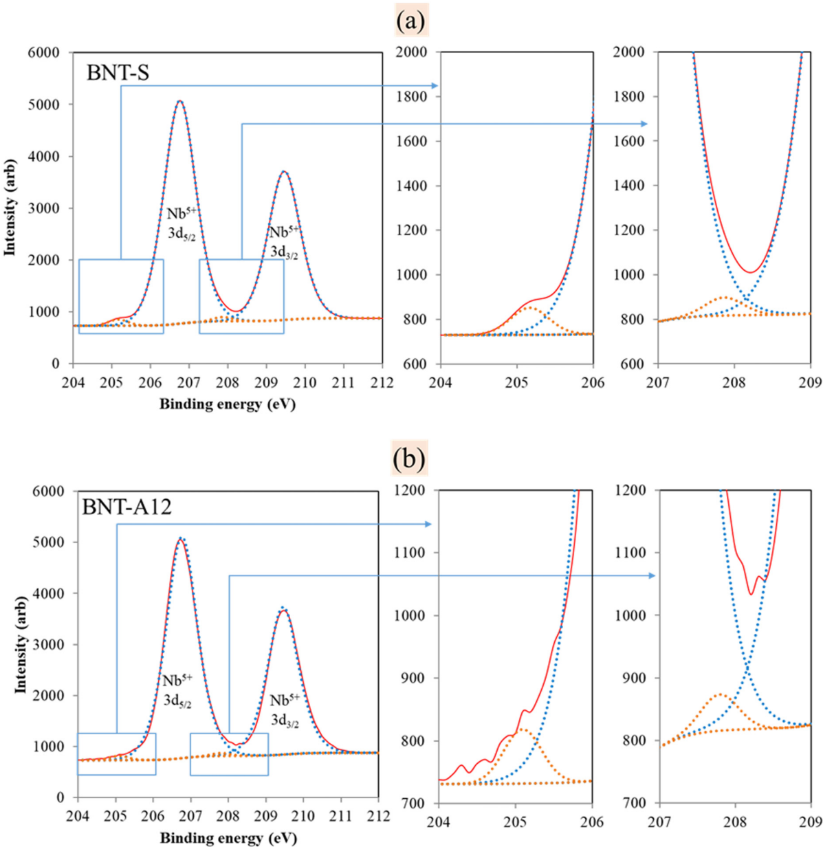
FIG. 8. (a) XPS spectra for air-sintered \text{Ba}_6\text{Ti}_2\text{Nb}_8\text{O}_{30} showing only the presence of \text{Nb}^{5+} and (b) XPS spectra for BTN-A12 showing the presence of both \text{Nb}^{5+} and \text{Nb}^{4+} .
