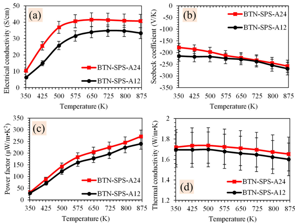
FIG. 11. Temperature dependence of thermoelectric properties of SPS-prepared \text{Ba}_6\text{Ti}_2\text{Nb}_8\text{O}_{30} samples annealed in the reducing atmosphere. (a) Electrical conductivity, (b) Seebeck coefficient, (c) power factor, and (d) thermal conductivity.
