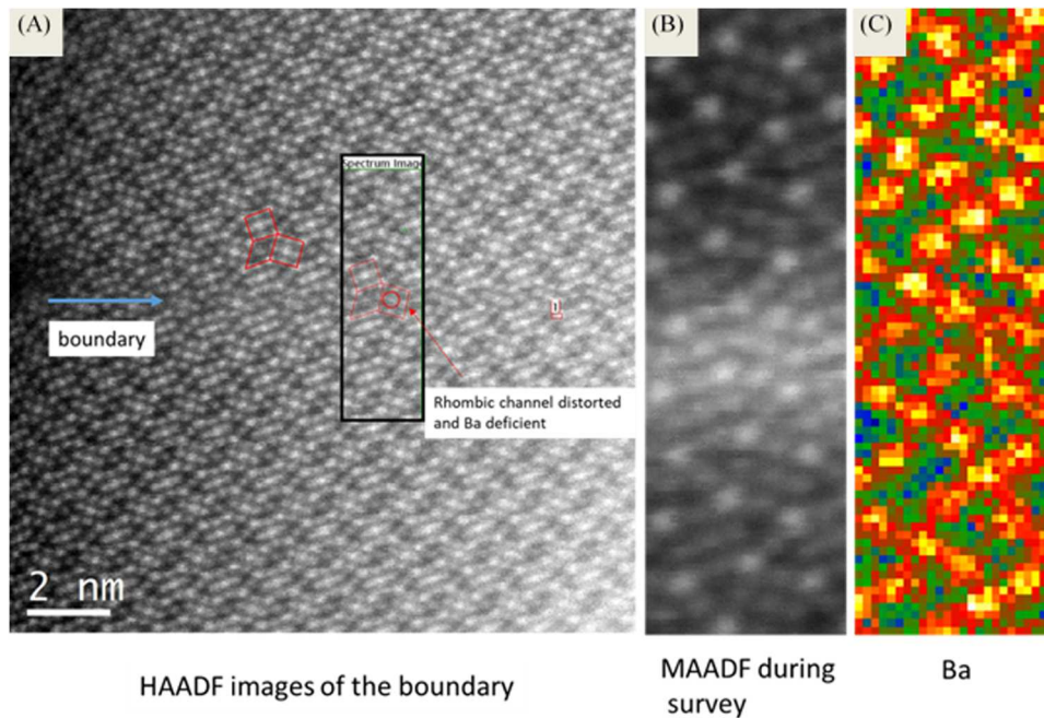
FIG. 6. [001] HAADF-EELS data for the linear defect in sample BTN-A12 (see Fig. 5). (a) HAADF image, (b) MADF image during data collection, and (c) Ba EELS map.
