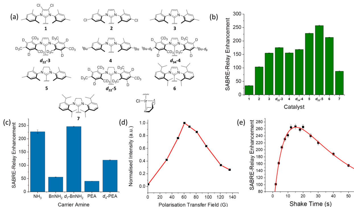
Figure 6 - (a) Structures of the ten different catalysts used in collecting the SABRE-Relay 13 C signal enhancements for D-glucose- 13 C 6 -d 7 shown in (b); the largest enhancement was observed for d 22 -5 , (c) Corresponding 13 C signal enhancement factors achieved using pre-catalyst d 22 -5 and the indicated NH containing materials ammonia (NH 3 ), benzylamine (BnNH 2 ), benzyl-d 7 -amine (d 7 -BnNH 2 ), phenethylamine (PEA) and phenethyl-1,1,2,2-d 4 -amine (d 4 -PEA); all samples contained 10.3 mM of the NH source and 4.8 mM of d 22 -5 in a DCM-d 2 : DMF (1.6:1) solution that was shaken at 60.6 G for ten seconds. (d) Polarization transfer field dependence on the signal gain for a D-glucose- 13 C 6 -d 7 sample with 4.8 mM of 3 in a DCM-d 2 : DMF (1.6:1) solution measured at 1 T; PTF obtained using a set of bespoke Halbach arrays. 69 (e) Signal gain as a function of shake time for a D-glucose- 13 C 6 -d 7 sample using 4.8 mM of d 22 -5 in a DCM-d 2 : DMF (1.6:1) solution; a bi-exponential equation was used to fit the data which highlights the process of polarization build up versus p-H 2 consumption in the NMR tube.
