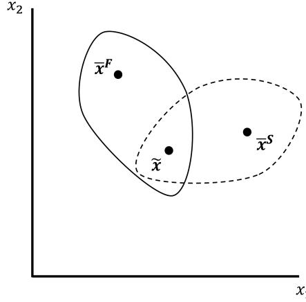
Figure 4: No identity conflict with overlapping quasi-norms
