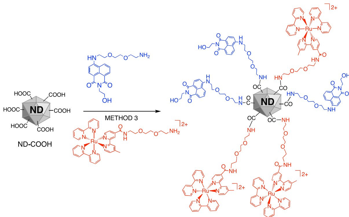
Figure 8. Cartoon representation of the synthetic route to co-functionalized ND decorated with naphthalimide (blue) and ruthenium (red) chromophores.
