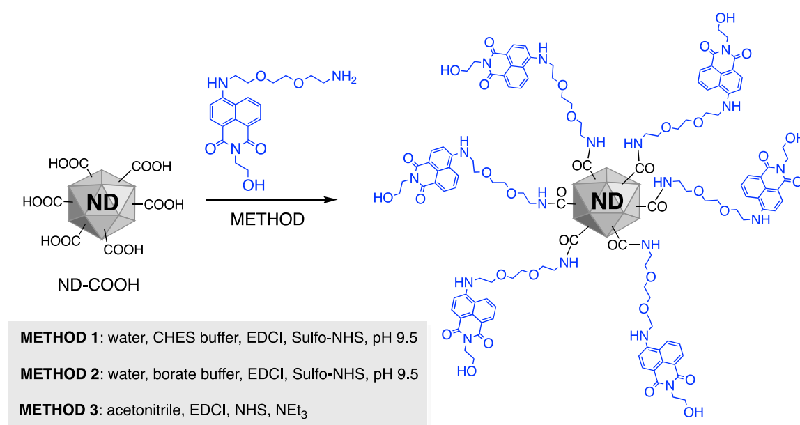
Figure 3. Cartoon representation of the synthetic routes to surface functionalized nanodiamond.
