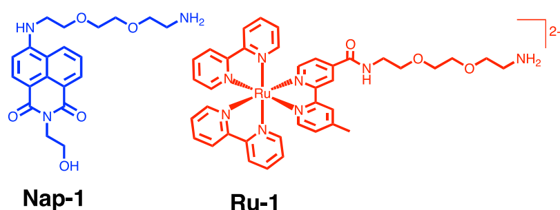
Figure 2. Structures of the amine terminated luminophores used to functionalize the surface of ND particles.
