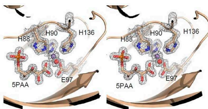
Figure 5. A stereo representation of the mF_{O}-DF_{C} electron density (grey mesh), contoured at 1.5\sigma , for the P132A, Y133G mutant PfPGI structure (mutant AG, PDB code: 4LUK), showing the manganese (purple sphere), coordinating water (red sphere), 5PAA and metal coordinating residues (sticks).
